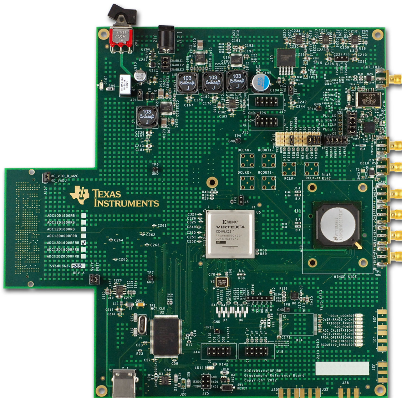
Figure 2. ADC1xDxxx(RF)RB Board Layout
