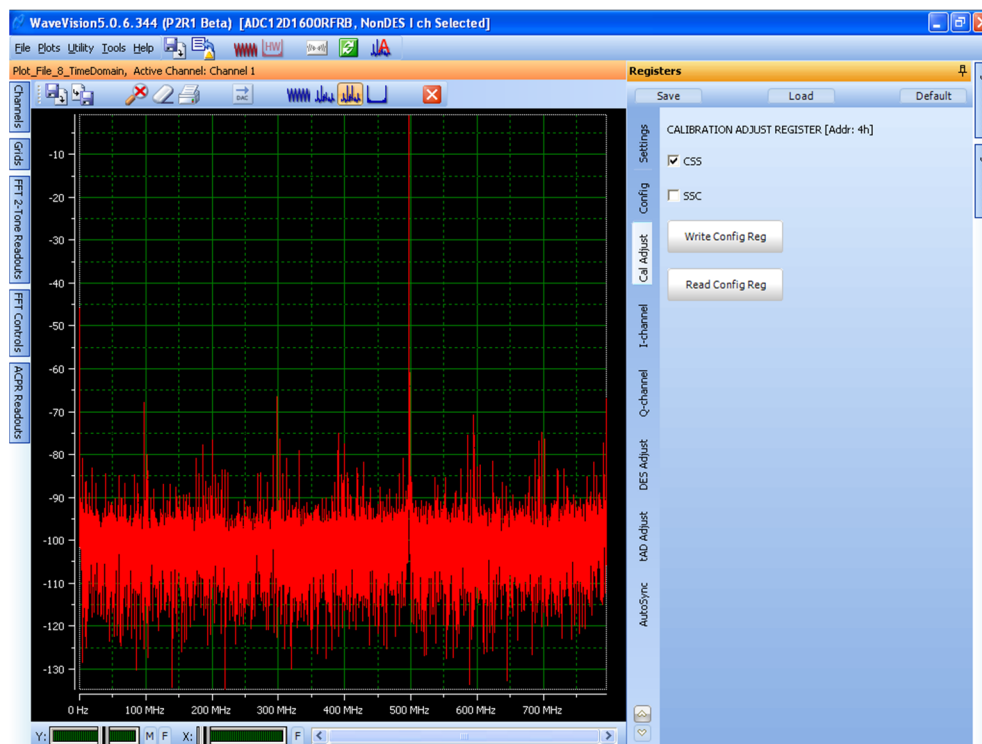
Figure 14. Cal Adjust Panel
