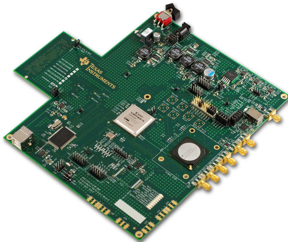
Figure 1. ADC1xDxxx_board1
