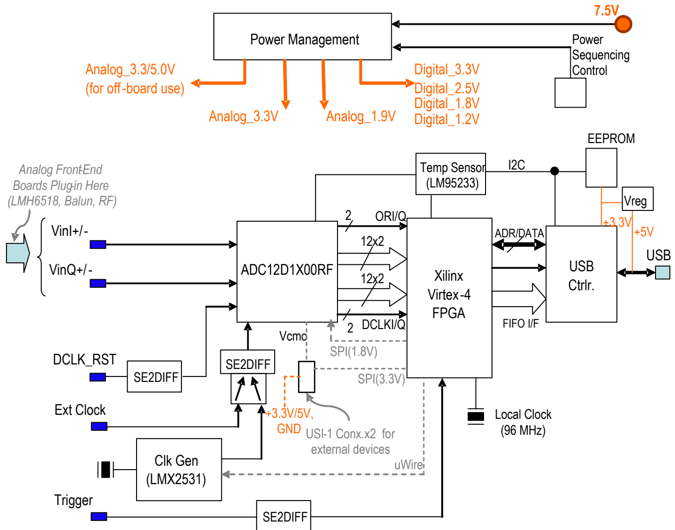
Figure 21. ADC1xDxxxx(RF)RB System Block Diagram
