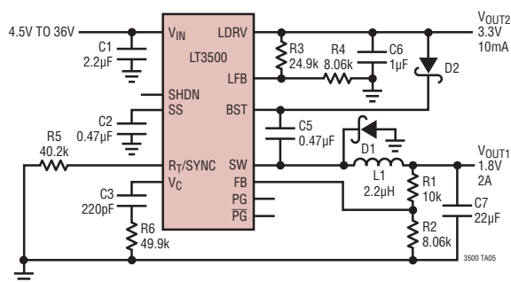
1.8V/2A Step-Down Regulator
