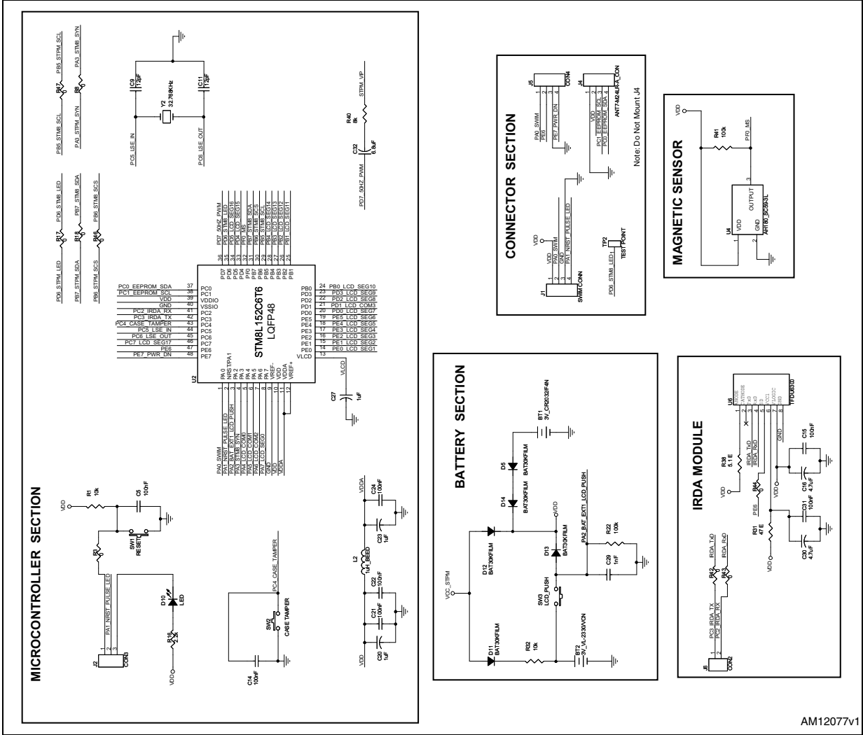
Figure 8. Schematics (1 of 2)
