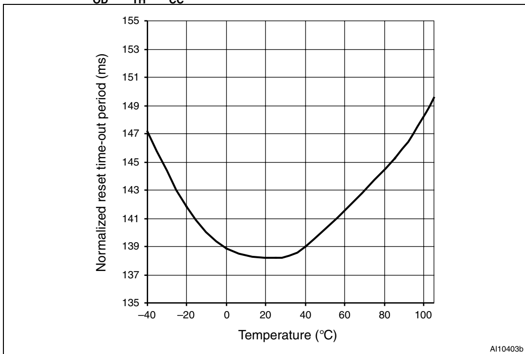
Figure 14. Normalized reset time-out period ( t_{\text{rec}} ) vs. temperature - V_{\text{OD}} = V_{\text{TH}} - V_{\text{CC}}
