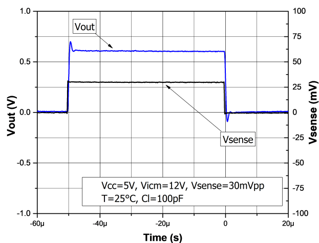
Figure 36. Small signal response with V_{CC} = 5\text{ V} (TSC2010)
