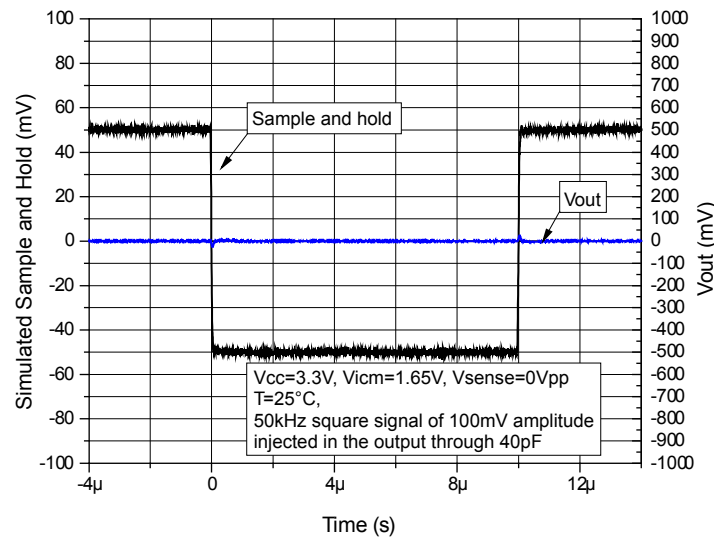
Figure 66. Capacitive load response at V_{CC} = 3.3 V with a step of 100 mV
