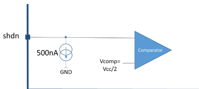
Figure 64. SHDN pin
