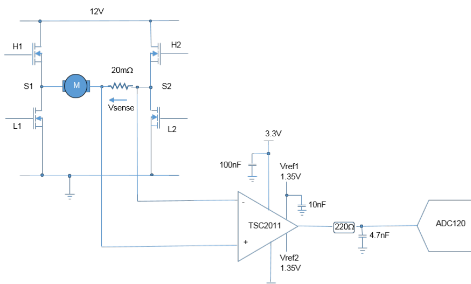
Figure 79. Half-bridge application
