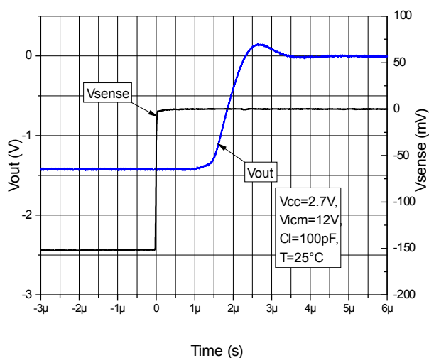
Figure 77. Negative overvoltage recovery V_{CC} = \pm 2.5 V
