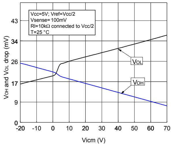
Figure 17. V_{OH} and V_{OL} vs. input common mode voltage with V_{CC} = 5\text{ V}
