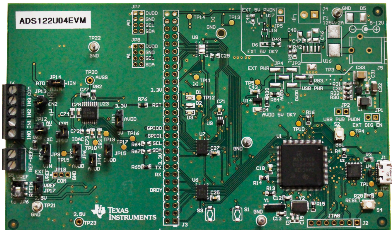
Figure 1. ADS1x2U04 Evaluation Module (ADS122U04EVM Shown)
