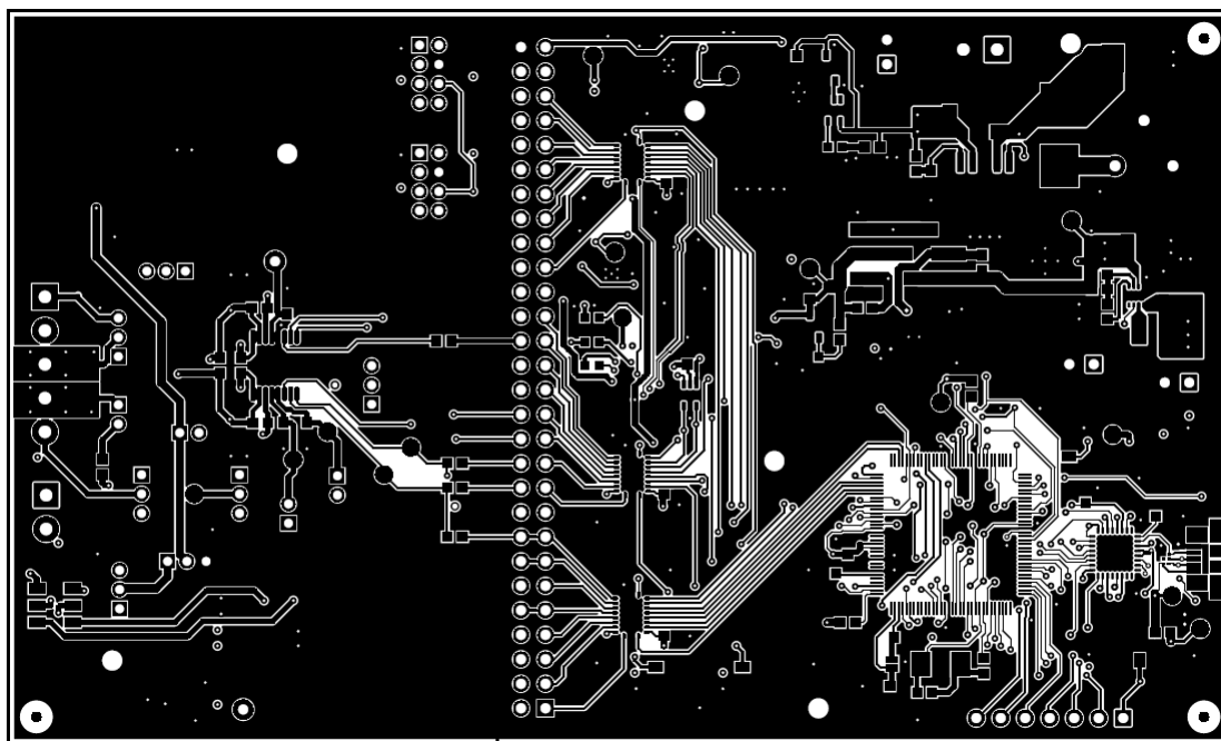
Figure 24. Top Layer (Positive)
