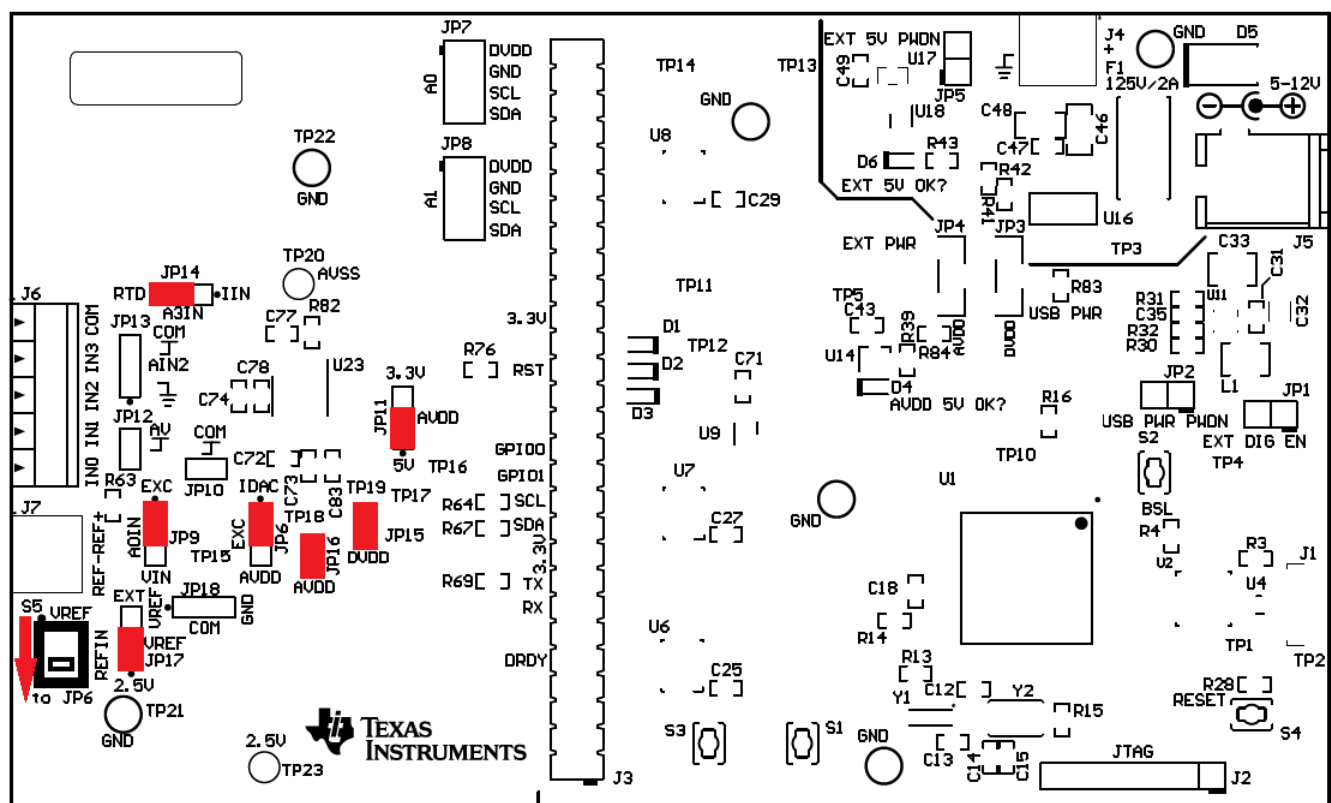
Figure 2. ADS1x2U04 EVM
