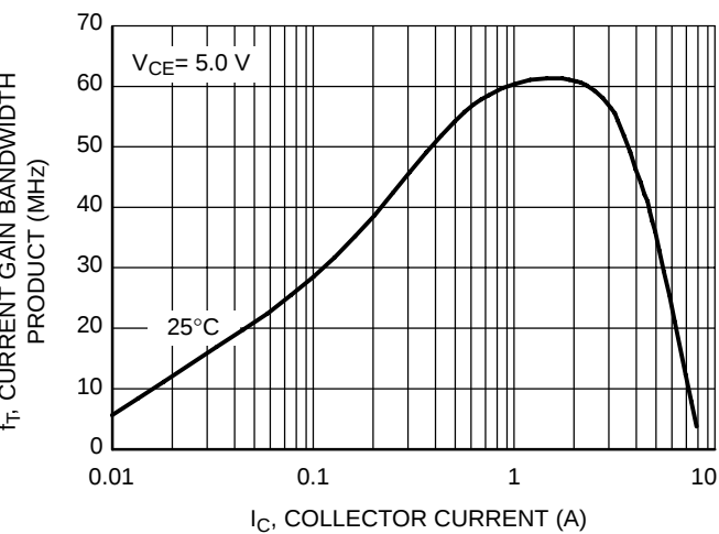
Figure 10. MJL0302A Current Gain Bandwidth Product
