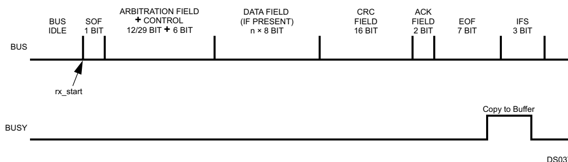
Figure 18-20. Receive Timing
