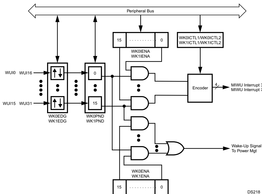
Figure 13-1. Multi-Input Wake-Up Module Block Diagram
