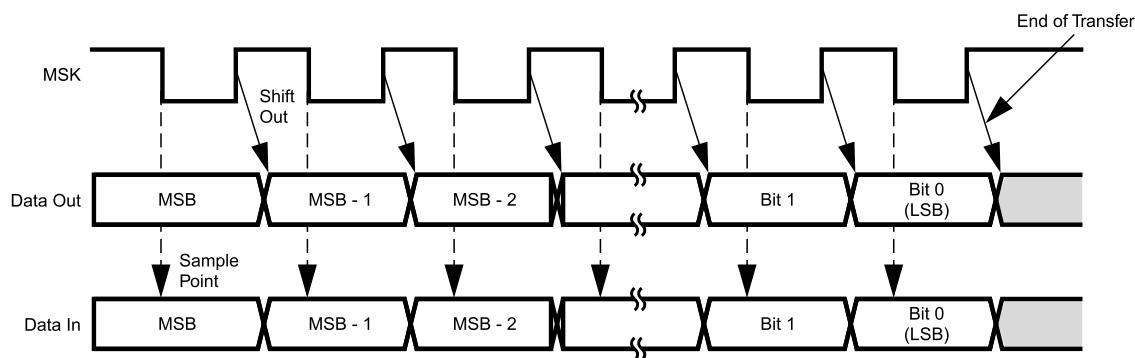
Figure 22-6. Alternate Mode (SCIDL = 1)
