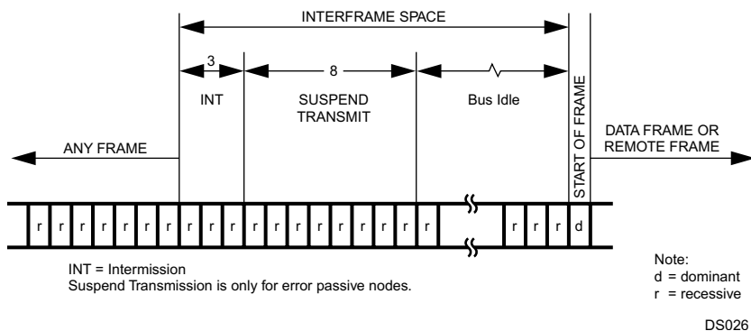
Figure 18-9. Interframe Space
