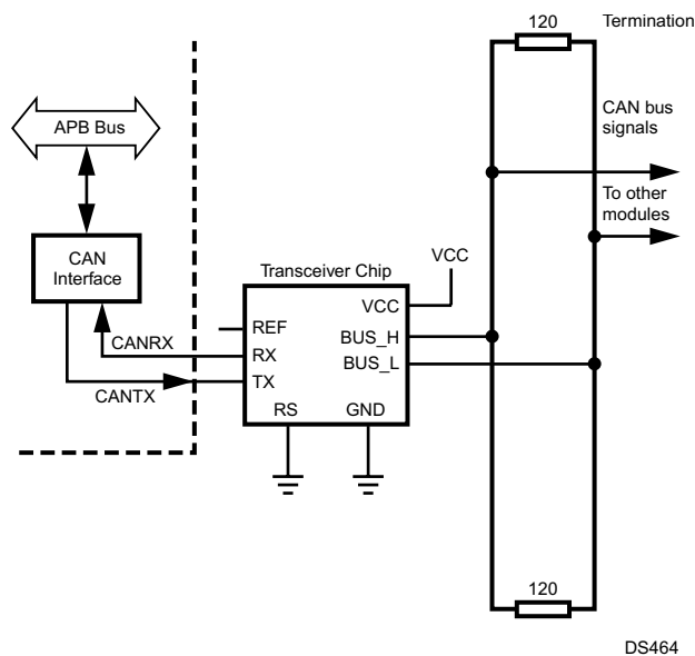
Figure 18-31. External Transceiver
