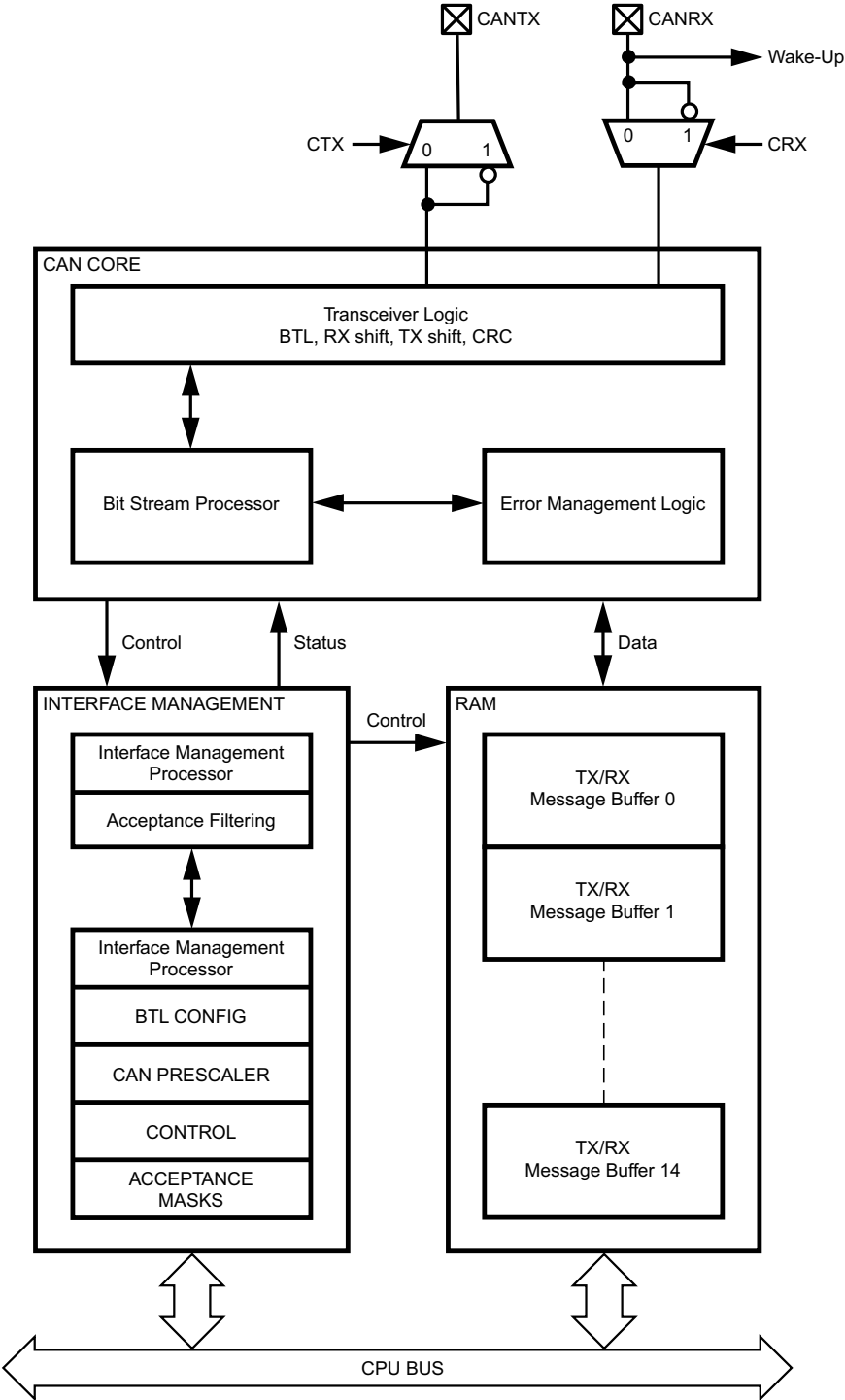
Figure 18-1. CAN Block Diagram
