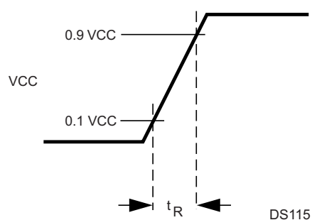
Figure 29-4. Power-On Reset
