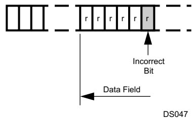
Figure 18-30. EBID Example
