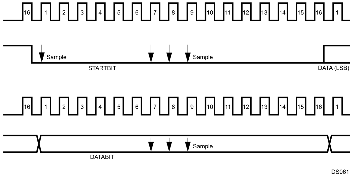
Figure 21-2. UART Asynchronous Communication
