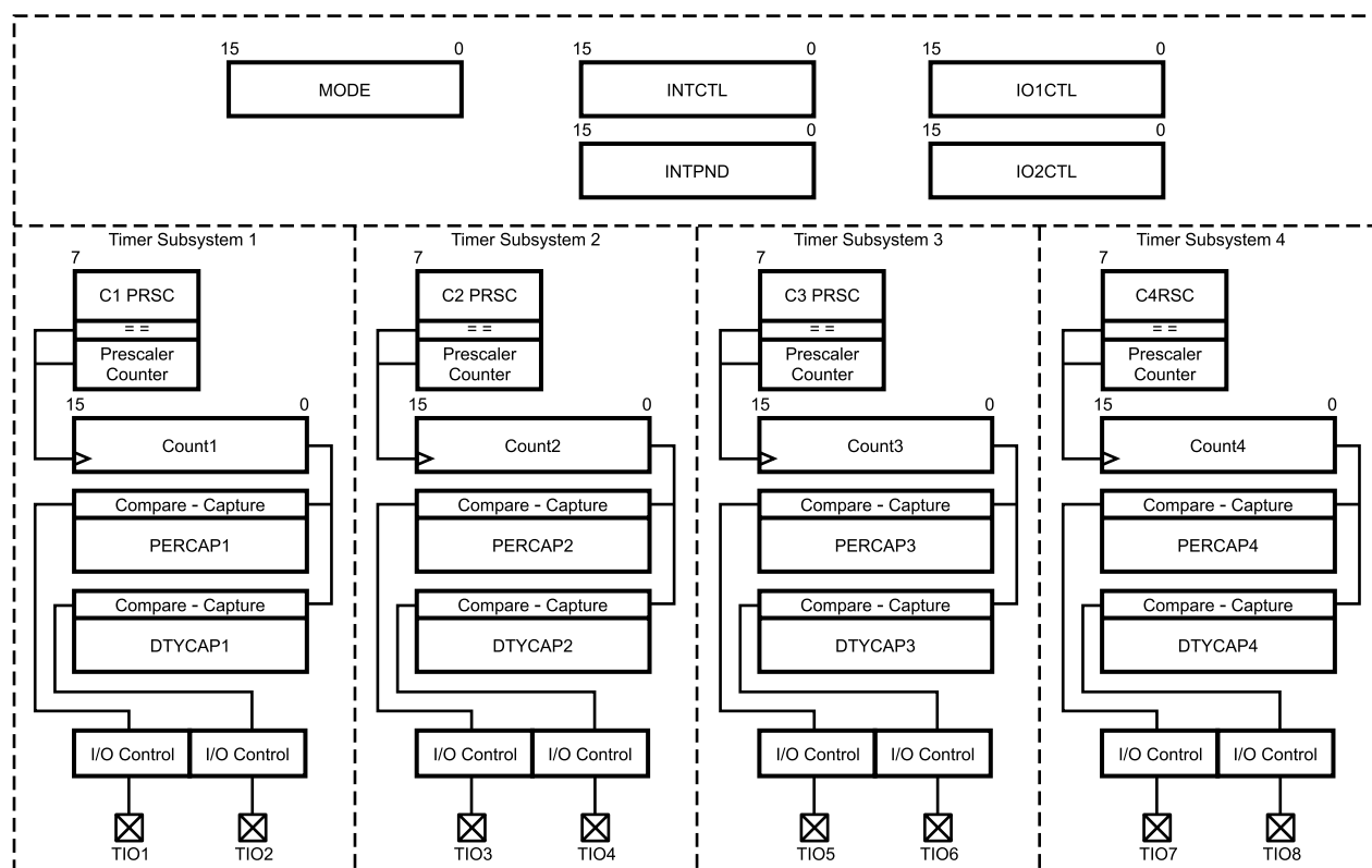
Figure 26-1. Versatile Timer Unit Block Diagram
