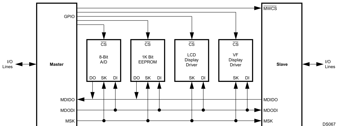
Figure 22-1. Microwire Interface
