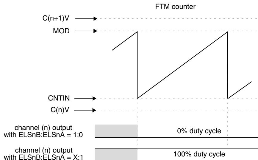
Figure 39-193. Channel (n) output if C(n)V and C(n+1)V are not between CNTIN and MOD
