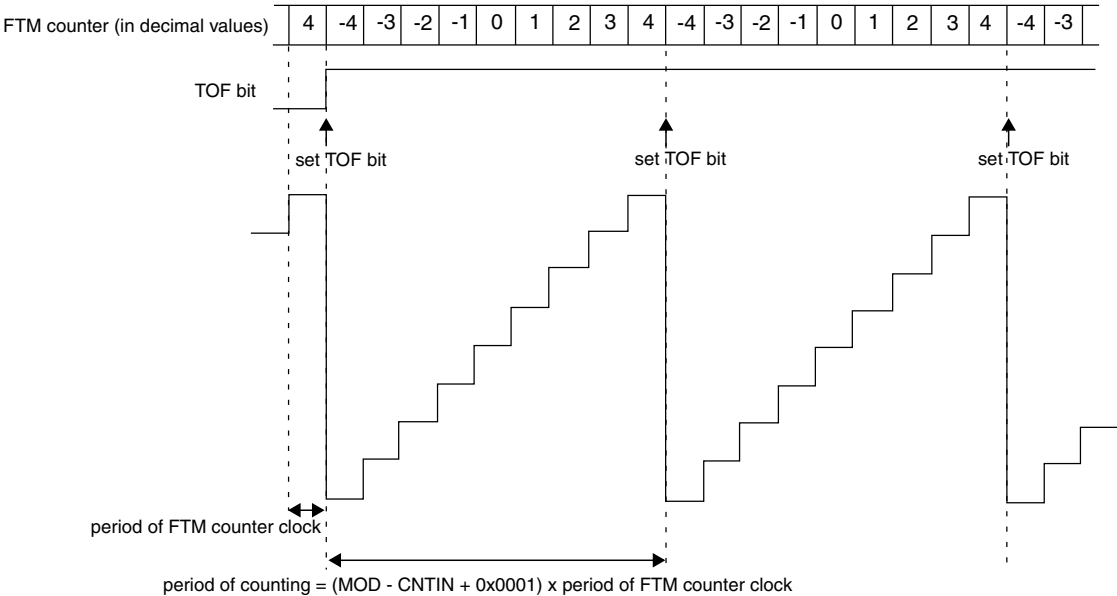
Figure 39-168. Example of FTM up and signed counting
