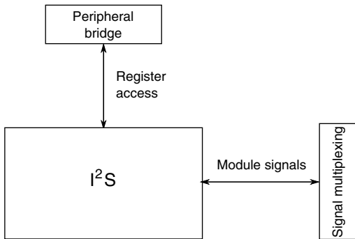
Figure 3-59. I²S configuration
