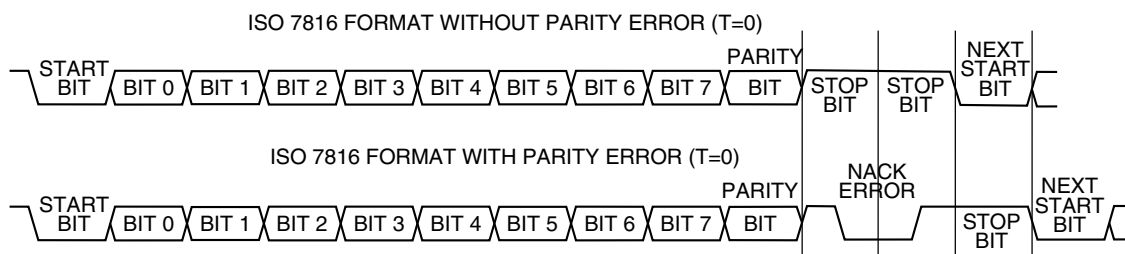
Figure 49-264. ISO-7816 T = 0 data format
