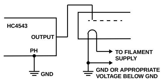
FIGURE 8. CONNECTION TO FLUORESCENT DISPLAY READOUT
