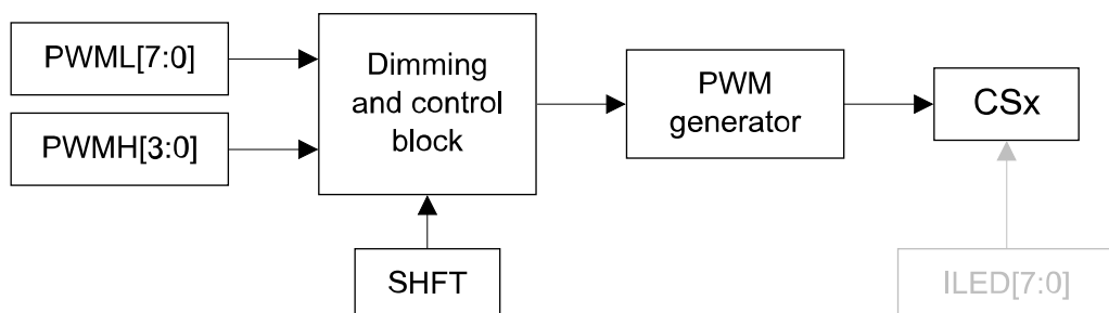
Figure 6. Digital dimming
