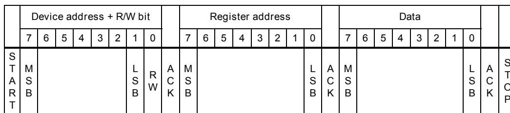
Figure 15. Interface protocol
