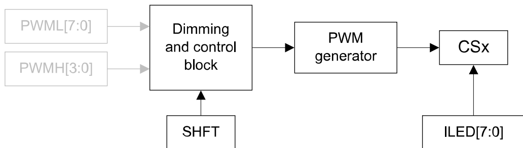
Figure 5. Analog dimming
