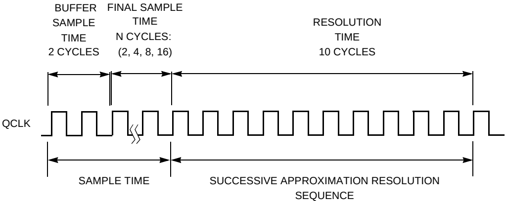
Figure 5-5 Conversion Timing
