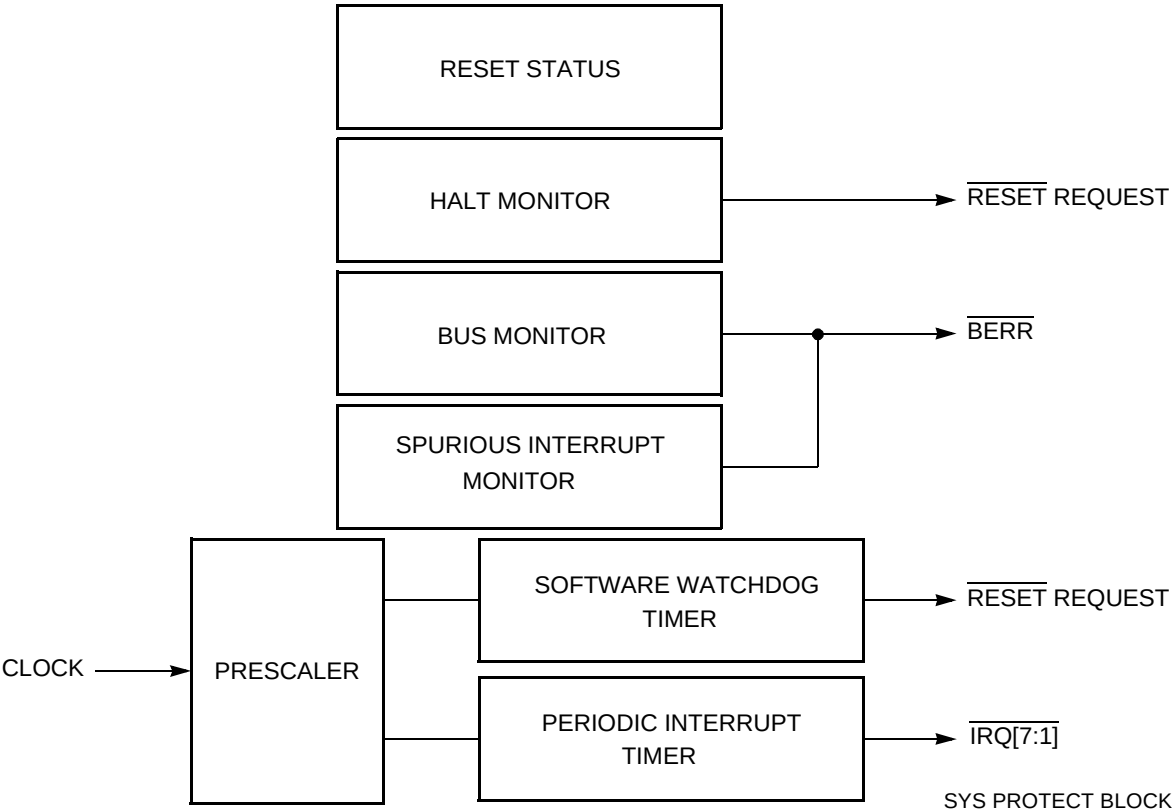
Figure 4-7 System Protection
