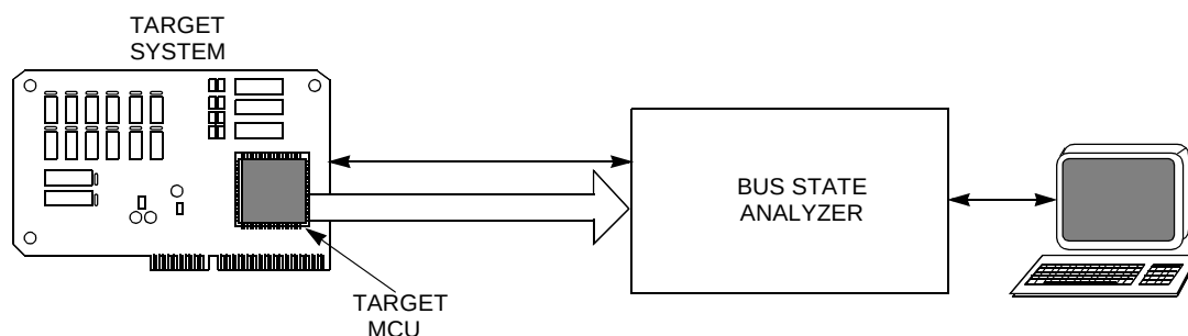
Figure 3-9 Bus State Analyzer Configuration
