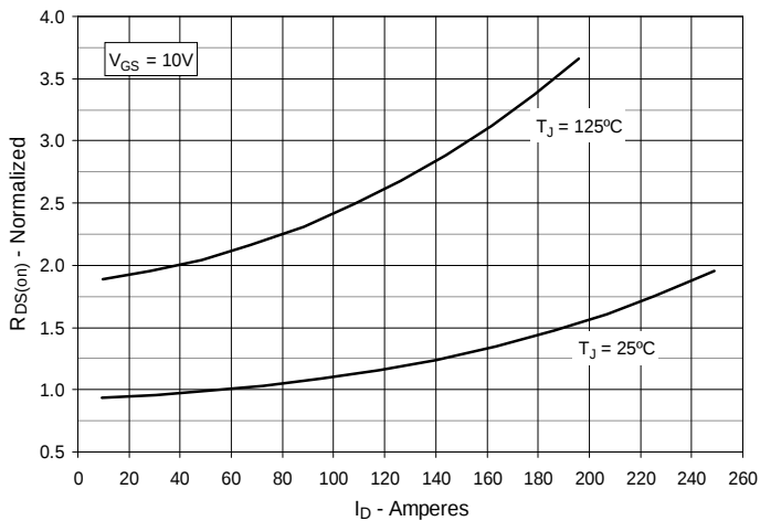
Fig. 5. R_{DS(on)} Normalized to I_D = 55A Value vs.
