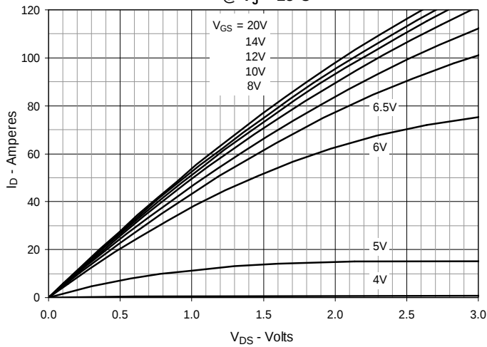
Fig. 3. Output Characteristics
