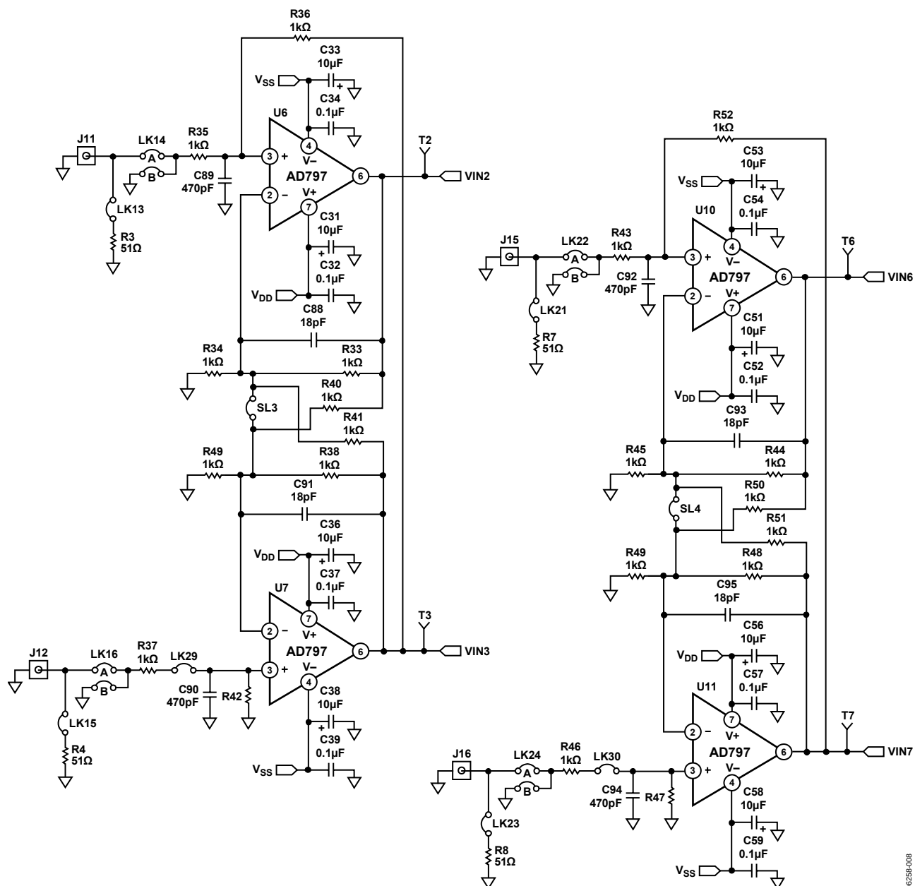
Figure 8. Schematic (Continued)
