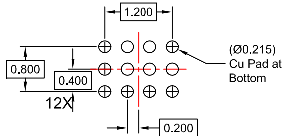
RECOMMENDED MOUNTING FOOTPRINT (NSMD PAD TYPE)
