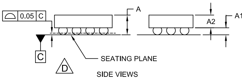
SIDE VIEWS
