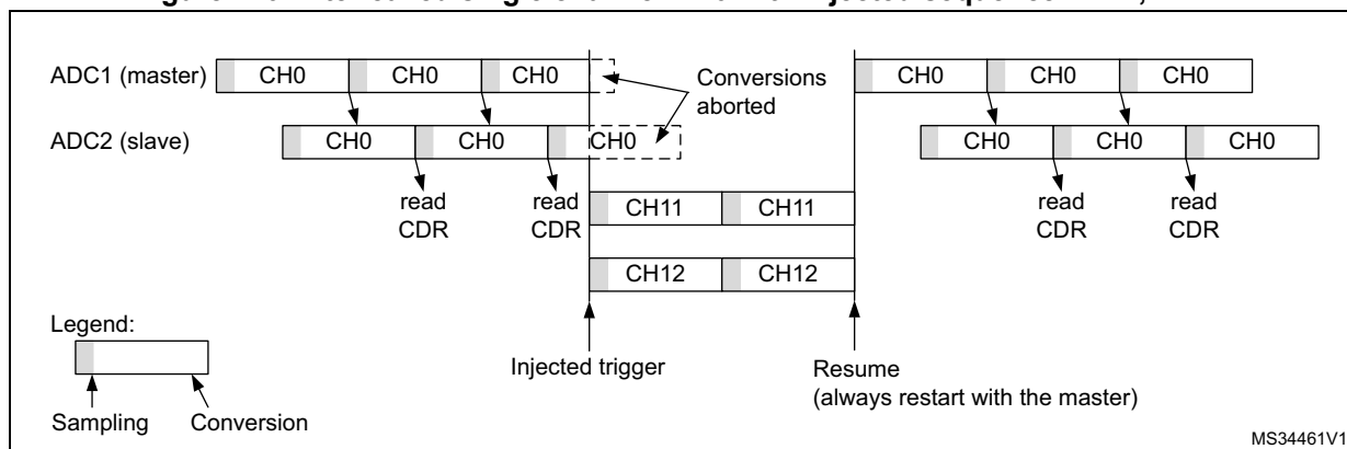
Figure 120. Interleaved single channel CH0 with injected sequence CH11, CH12
