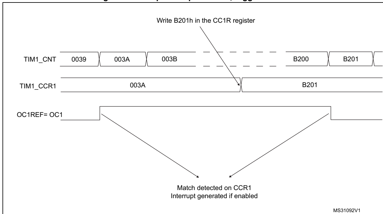
Figure 249. Output compare mode, toggle on OC1
