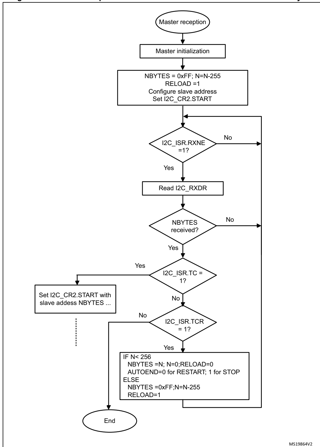
Figure 344. Transfer sequence flowchart for I2C master receiver for N &gt; 255 bytes
