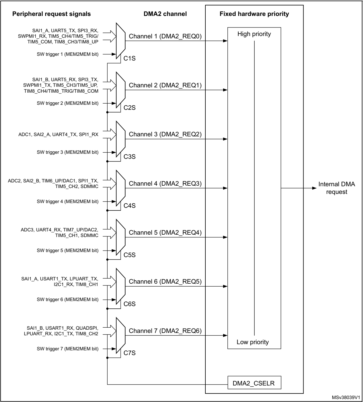
Figure 25. DMA2 request mapping
