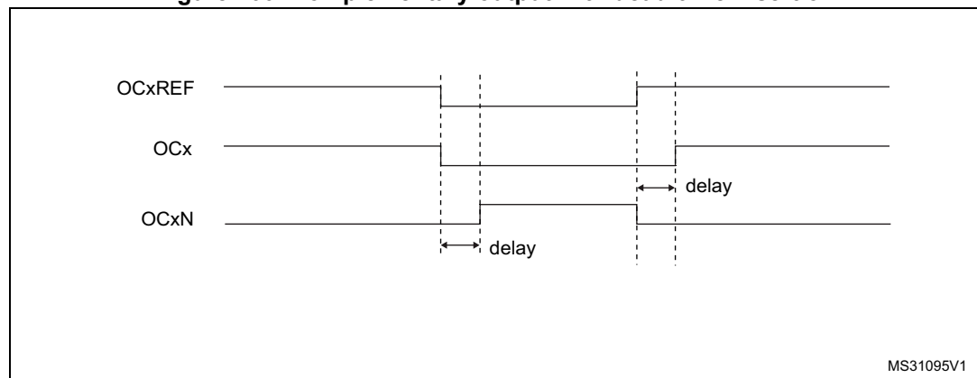
Figure 200. Complementary output with dead-time insertion
