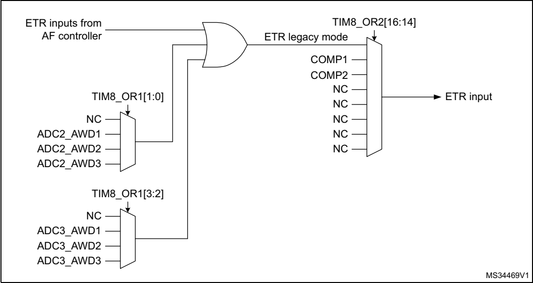
Figure 182. TIM8 ETR input circuitry
