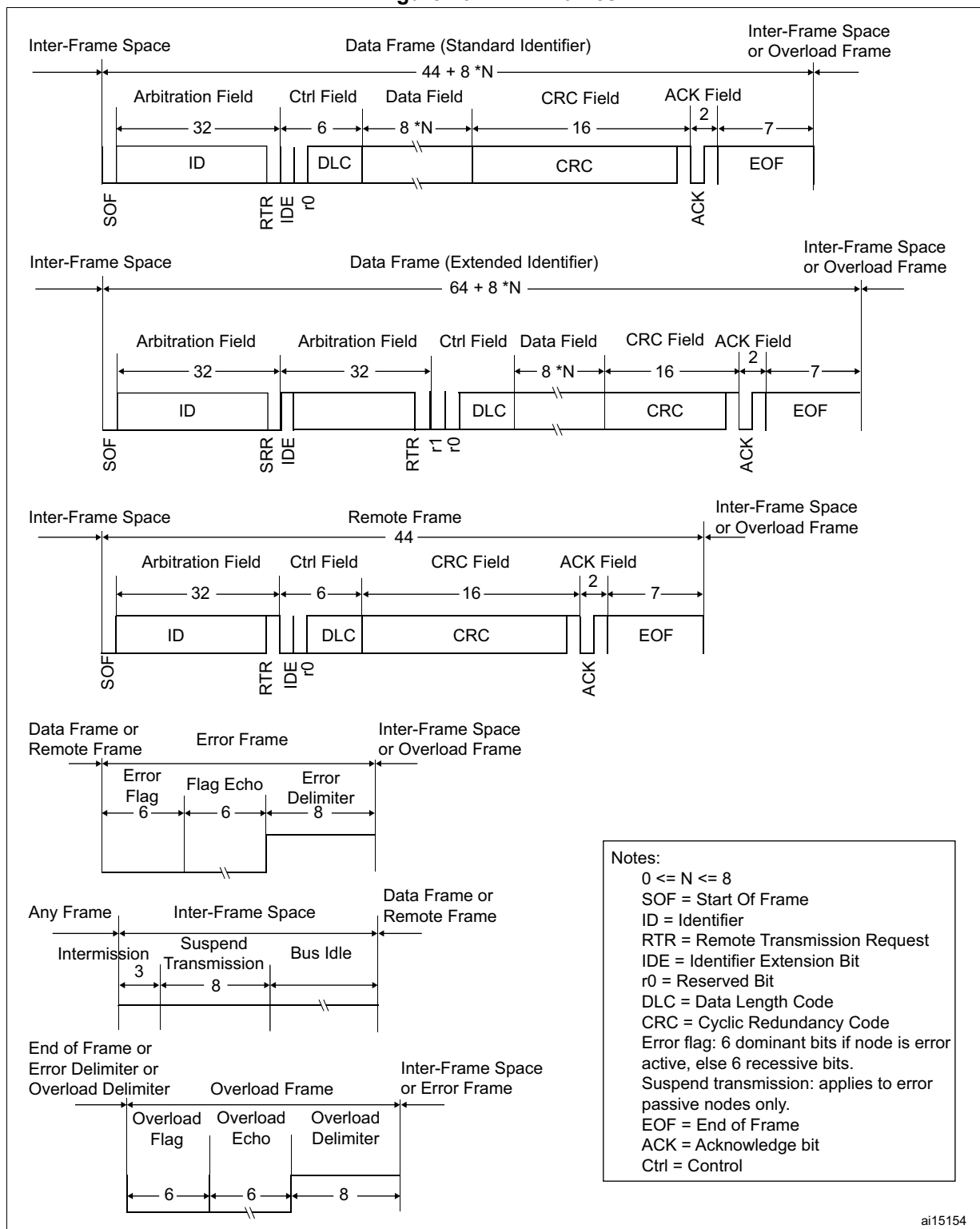
Figure 461. CAN frames
