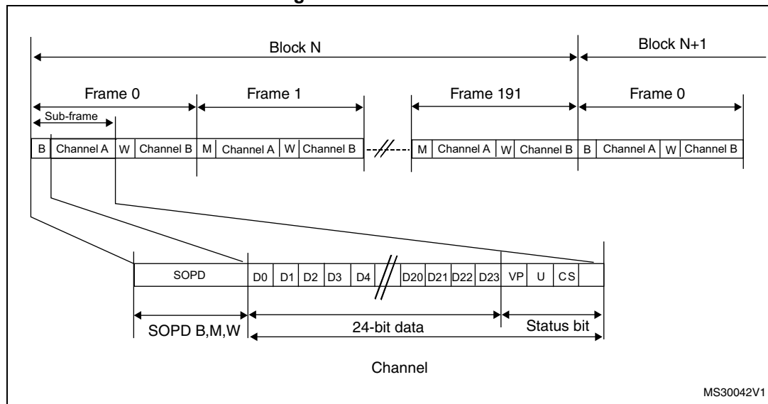
Figure 416. SPDIF format
