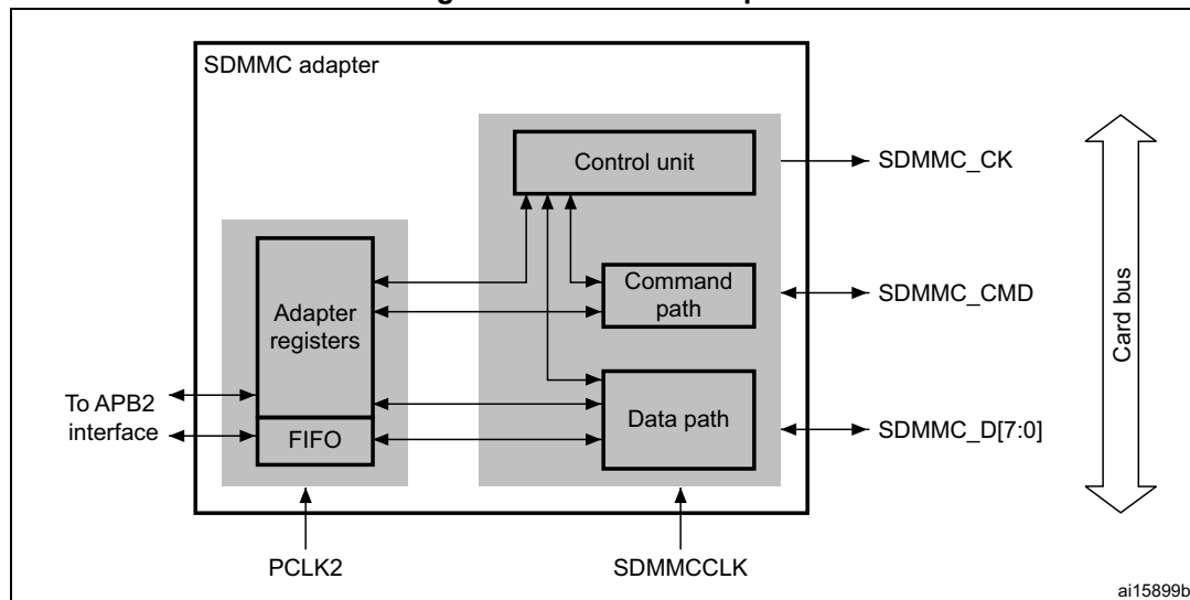
Figure 441. SDMMC adapter
