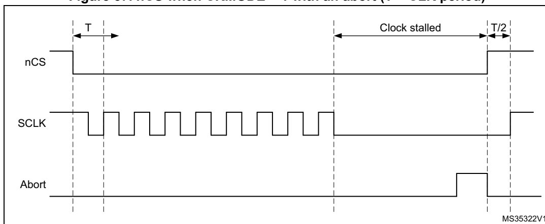
Figure 57. nCS when CKMODE = 1 with an abort ( T = \text{CLK period} )
