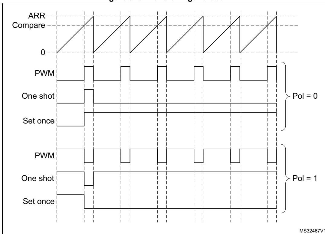
Figure 316. Waveform generation
