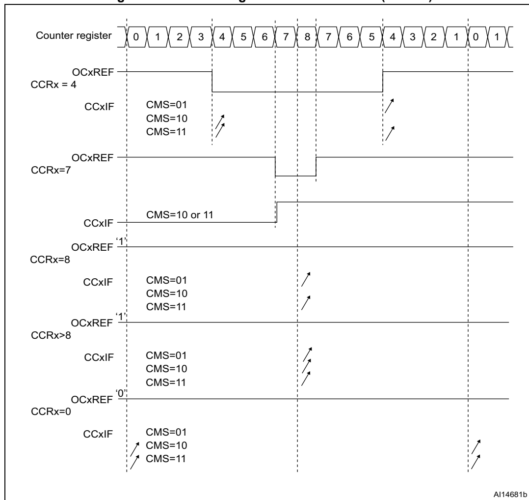
Figure 196. Center-aligned PWM waveforms (ARR=8)
