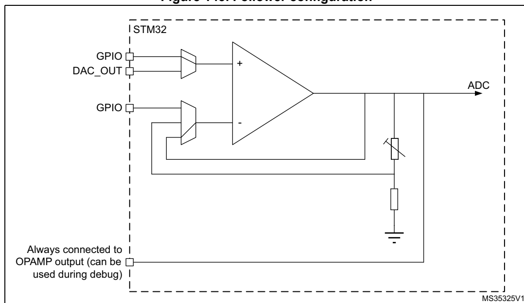
Figure 143. Follower configuration
