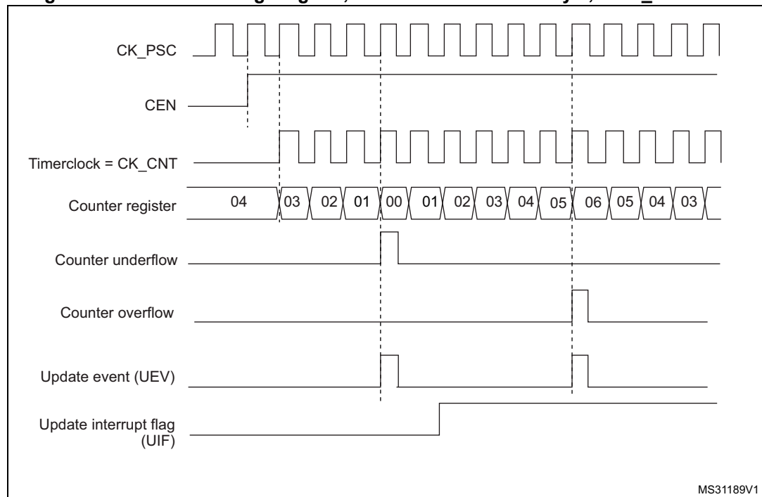
Figure 173. Counter timing diagram, internal clock divided by 1, TIMx_ARR = 0x6
