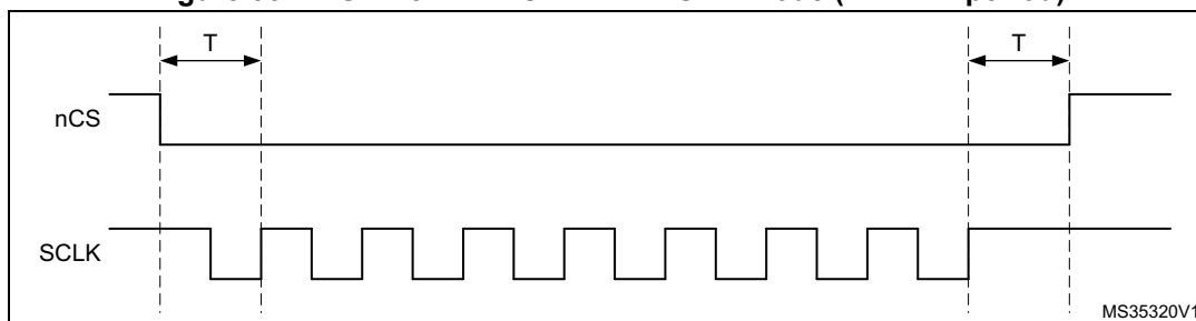
Figure 55. nCS when CKMODE = 1 in SDR mode ( T = \text{CLK period} )
