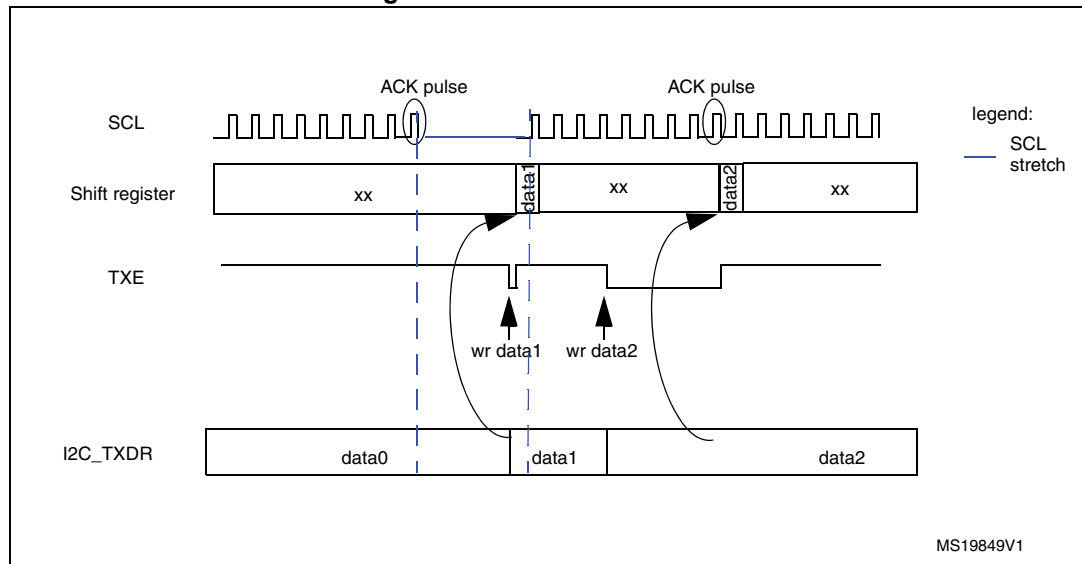
Figure 328. Data transmission
