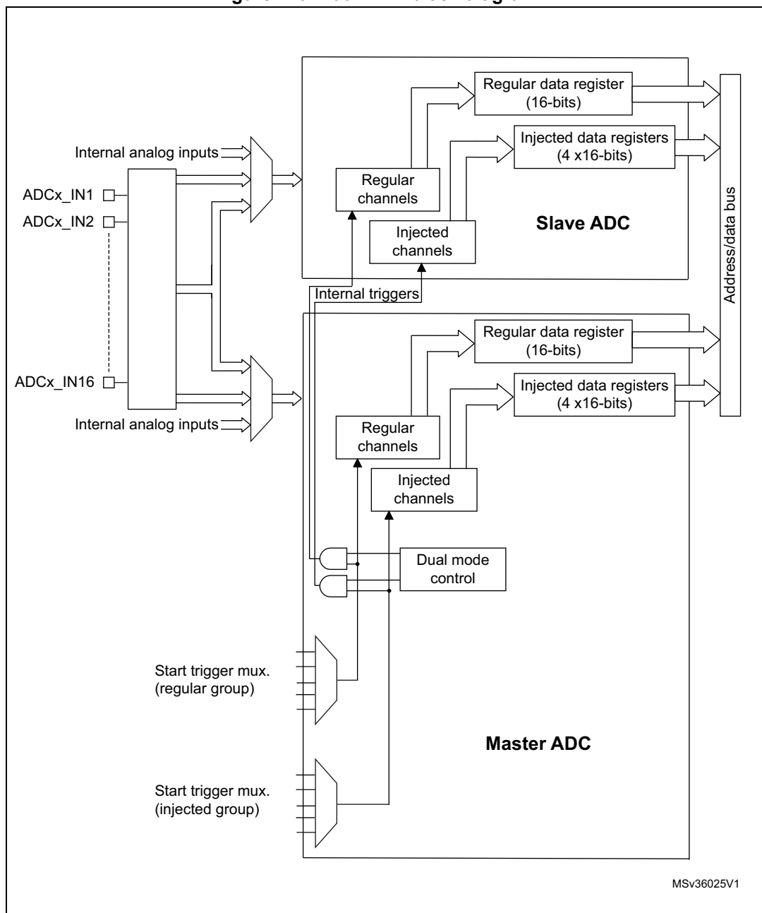
Figure 110. Dual ADC block diagram (1)
