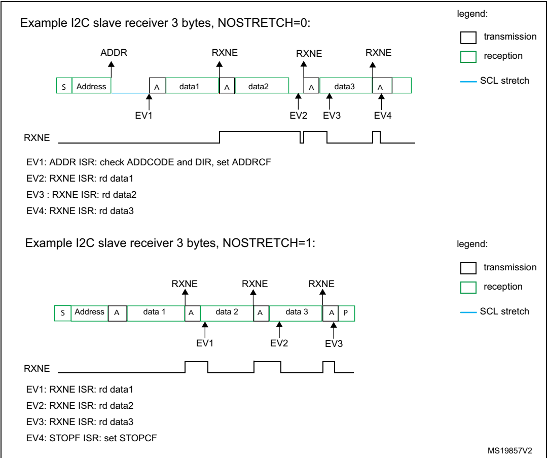
Figure 335. Transfer bus diagrams for I2C slave receiver
