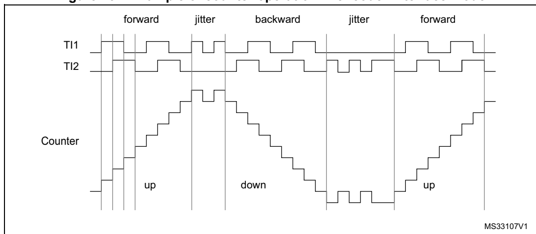
Figure 257. Example of counter operation in encoder interface mode
