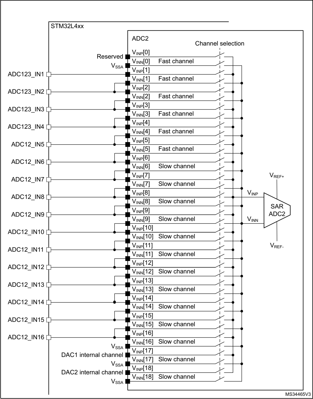
Figure 61. ADC2 connectivity
