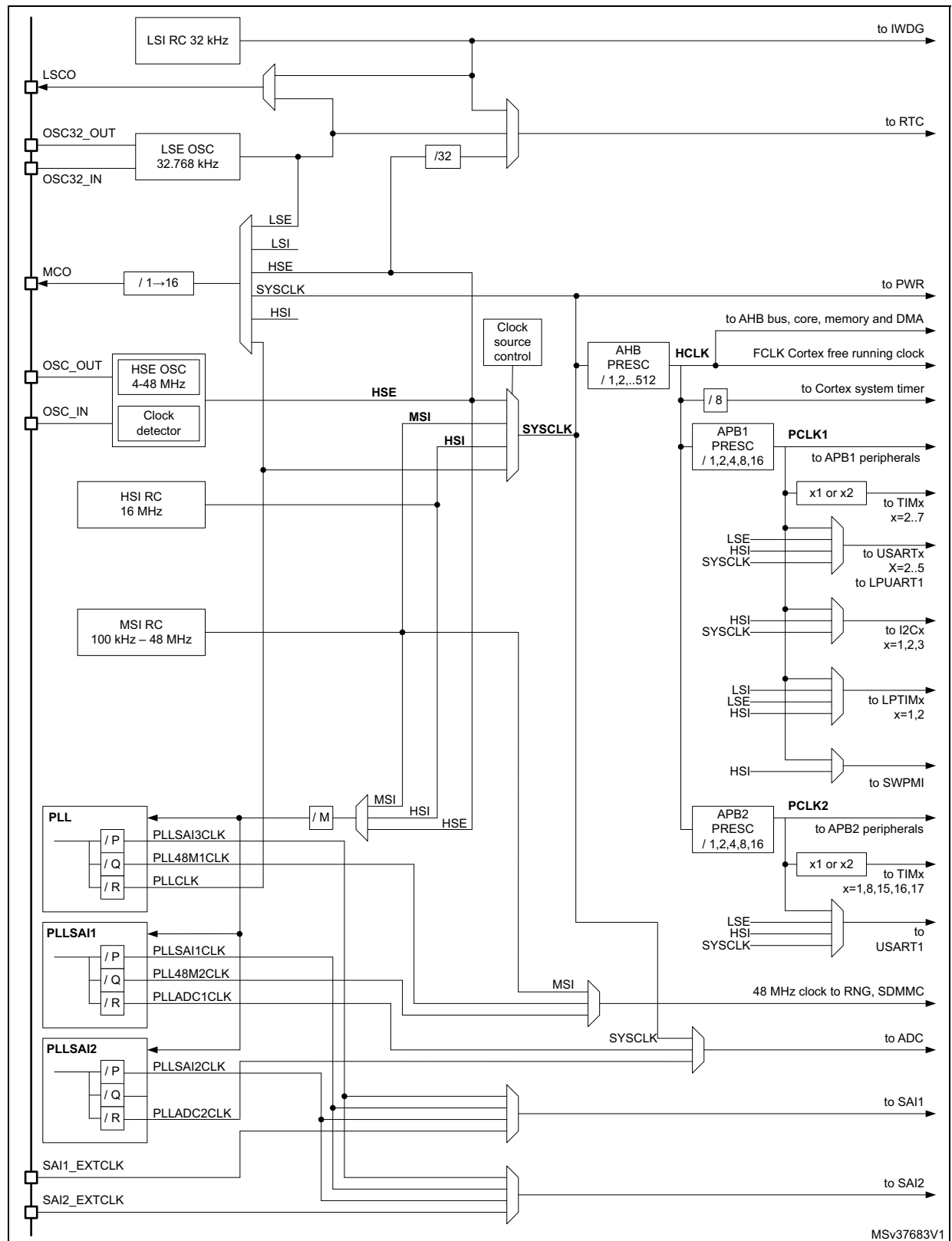
Figure 12. Clock tree
