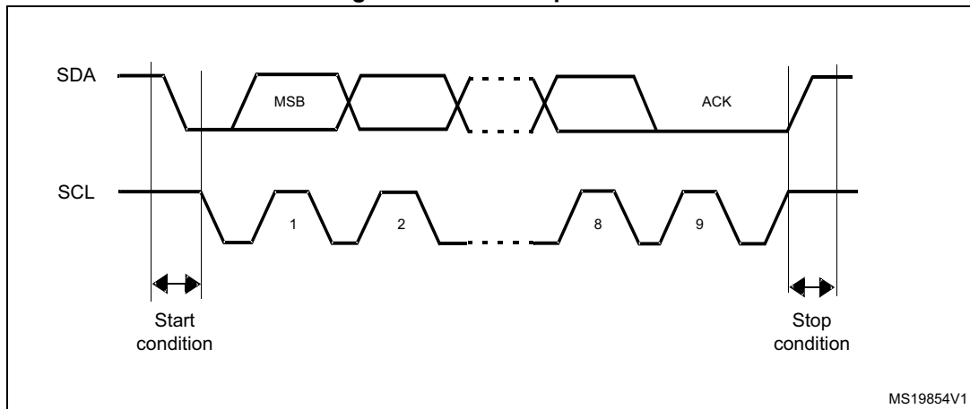
Figure 324. I 2 C bus protocol
