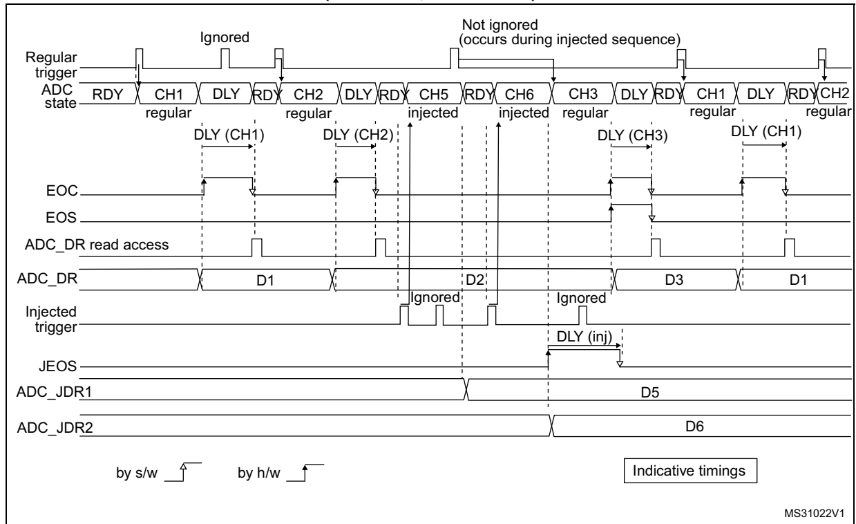
Figure 95. AUTODLY=1, regular HW conversions interrupted by injected conversions (DISCEN=1, JDISCEN=1)
