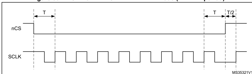
Figure 56. nCS when CKMODE = 1 in DDR mode ( T = \text{CLK period} )
