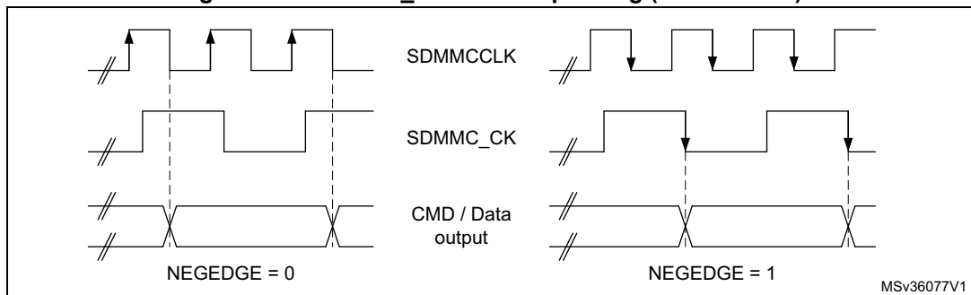
Figure 443. SDMMC_CLK clock dephasing (BYPASS = 0)
