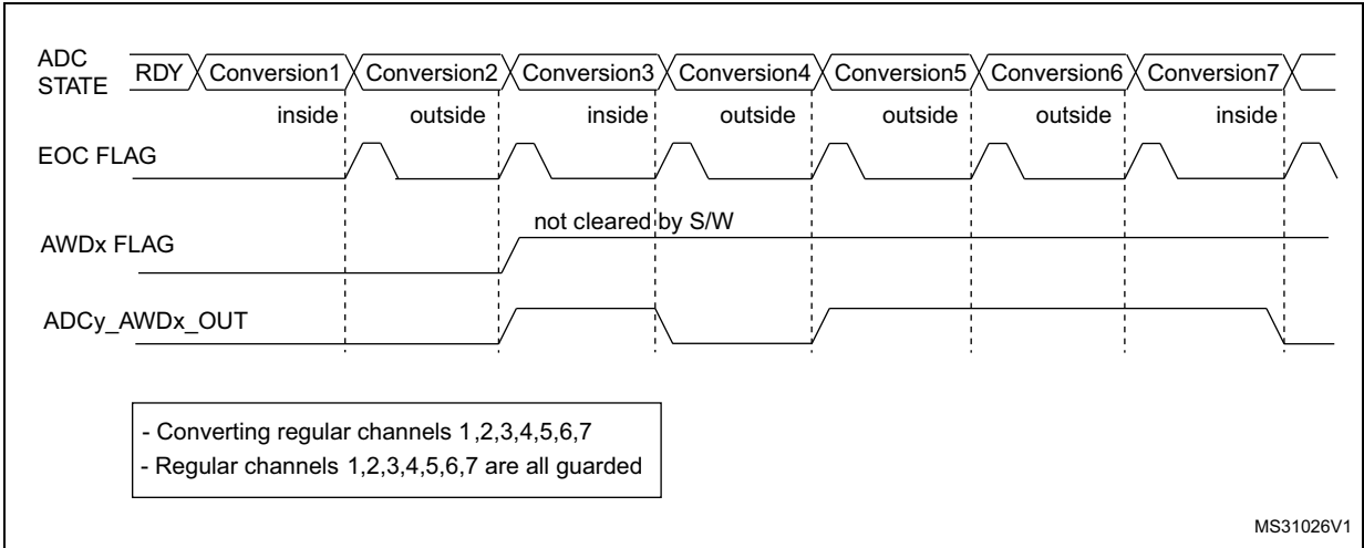
Figure 100. ADCy_AWDx_OUT signal generation (AWDx flag not cleared by SW)
