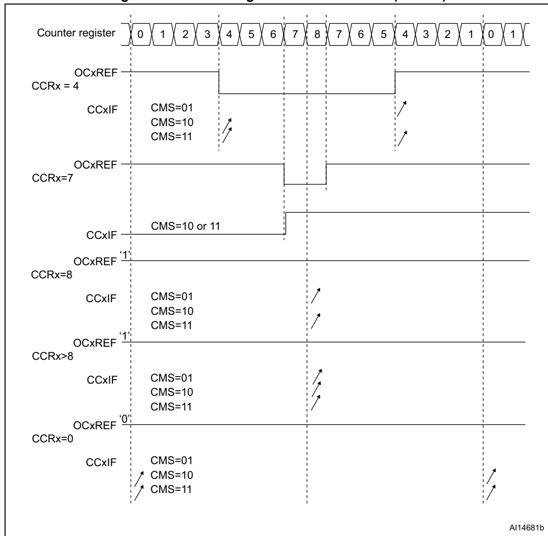
Figure 251. Center-aligned PWM waveforms (ARR=8)
