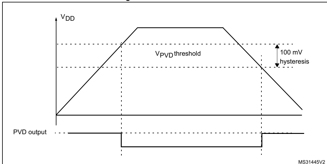
Figure 9. PVD thresholds
