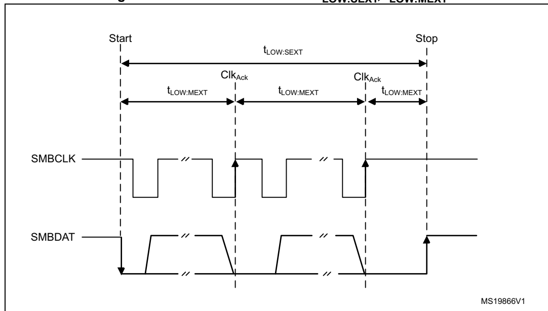
Figure 346. Timeout intervals for t_{\text{LOW:SEXT}} , t_{\text{LOW:MEXT}}
