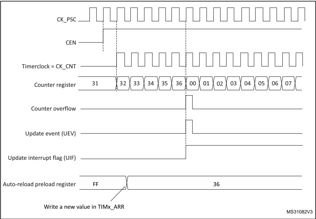
Figure 166. Counter timing diagram, update event when ARPE=0 (TIMx_ARR not preloaded)
