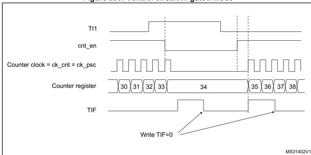
Figure 299. Control circuit in gated mode
