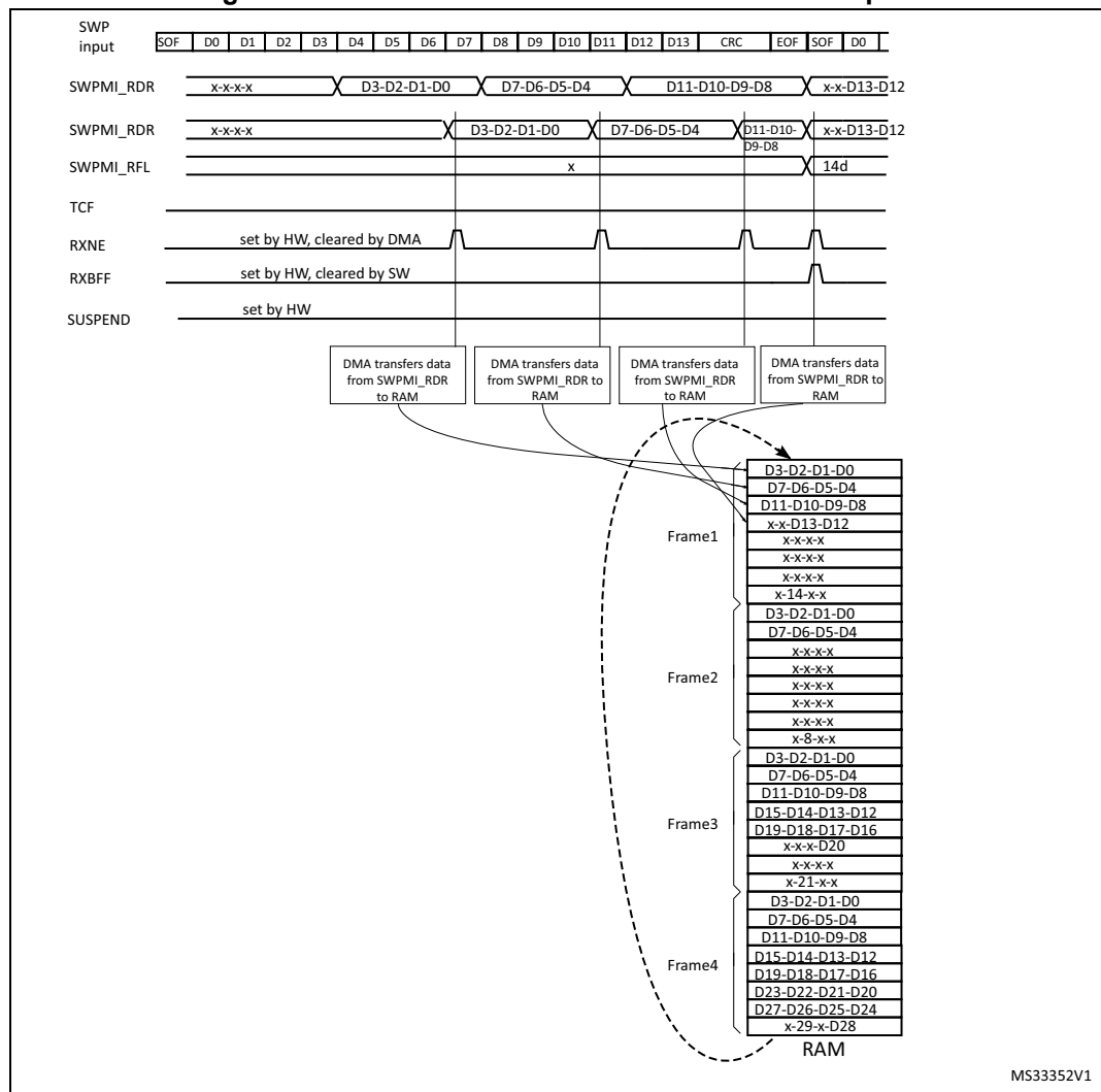
Figure 433. SWPMI Multi software buffer mode reception
