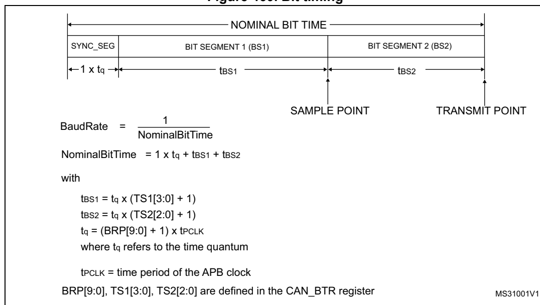
Figure 460. Bit timing
