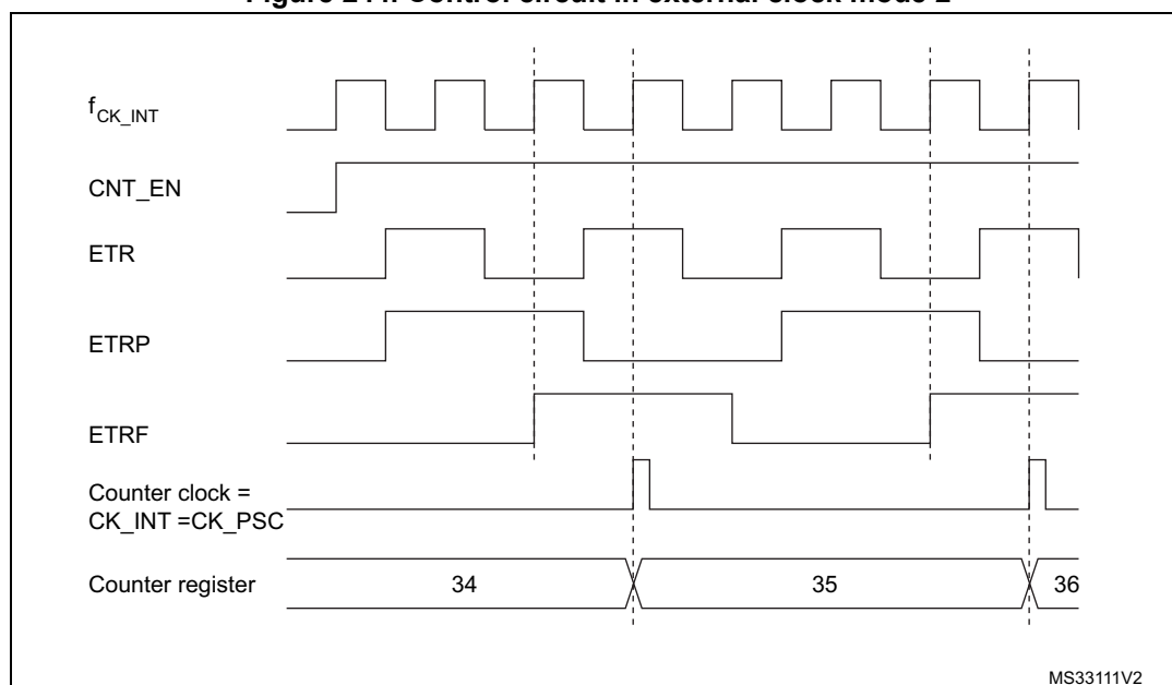
Figure 244. Control circuit in external clock mode 2
