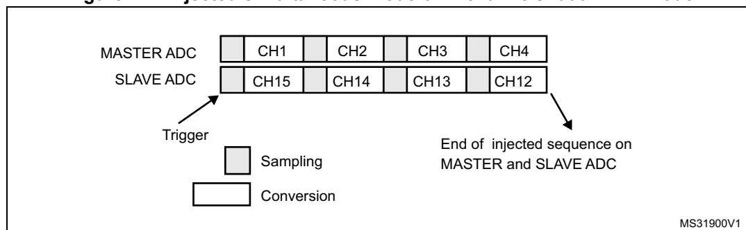
Figure 111. Injected simultaneous mode on 4 channels: dual ADC mode
