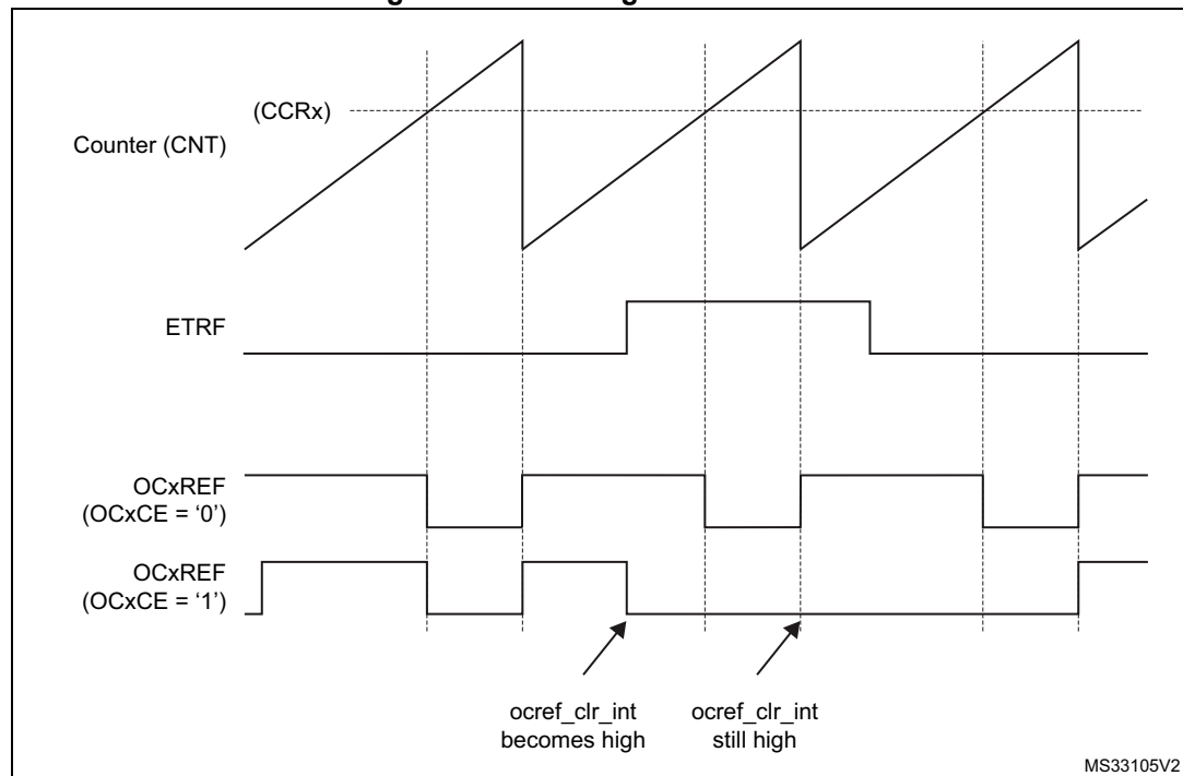
Figure 254. Clearing TIMx OCxREF
