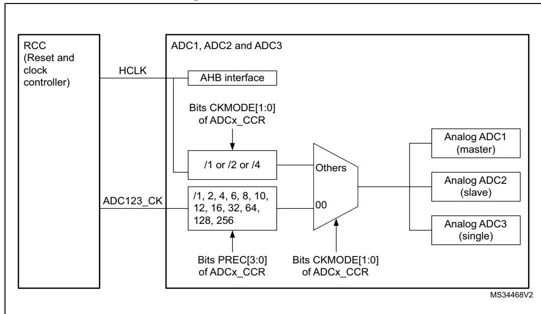
Figure 59. ADC clock scheme
