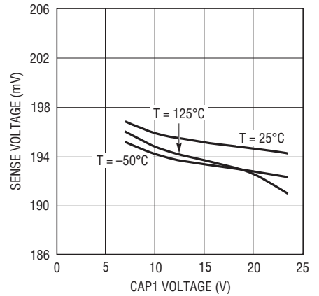
Sense Voltage (V CAP1 - V LED1 ) vs V CAP1
