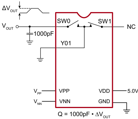
Charge Injection
