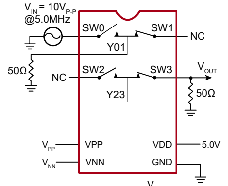
Crosstalk
