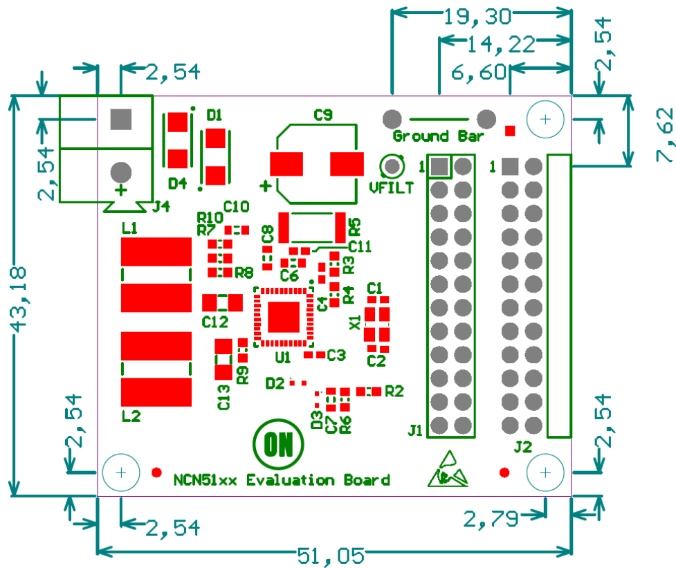
Figure 5.PCB Dimensions
