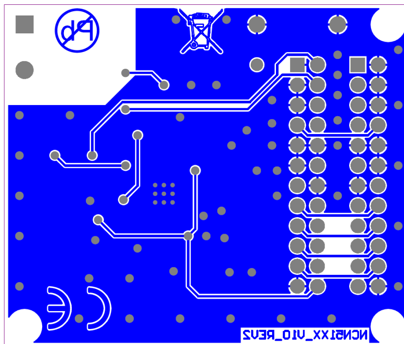
Figure 4.Bottom Layer Layout
