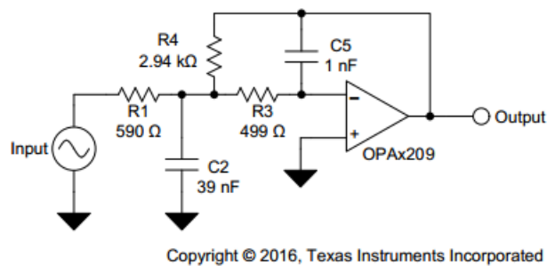
Figure 35. Low-Pass Filter
