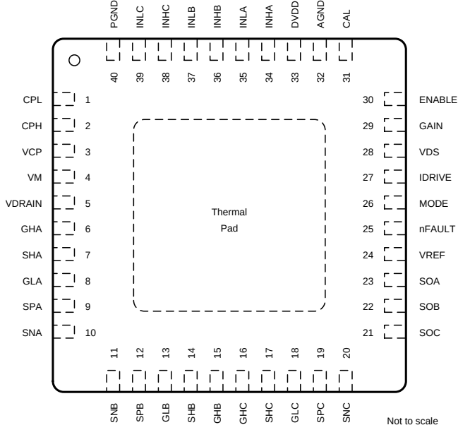
DRV8323H RTA Package 40-Pin WQFN With Exposed Thermal Pad Top View
