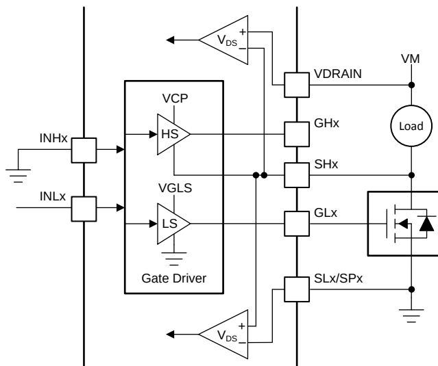
Figure 22. One Low-Side Driver
