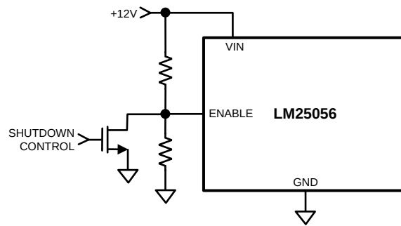
Figure 16. ENABLE Control
