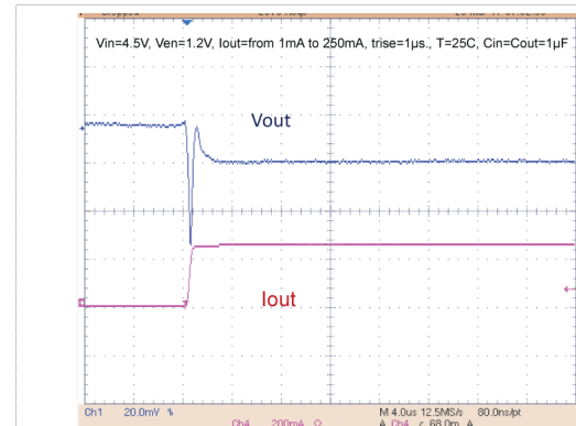
Figure 24. Load transient
