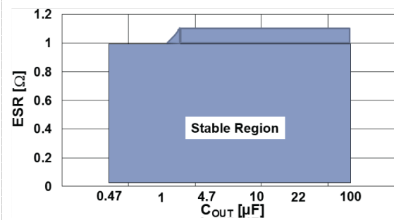
Figure 20. Stability region vs. C OUT and ESR
