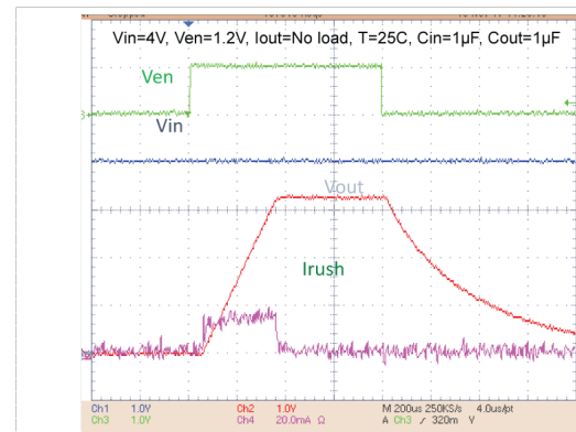
Figure 26. Inrush current
