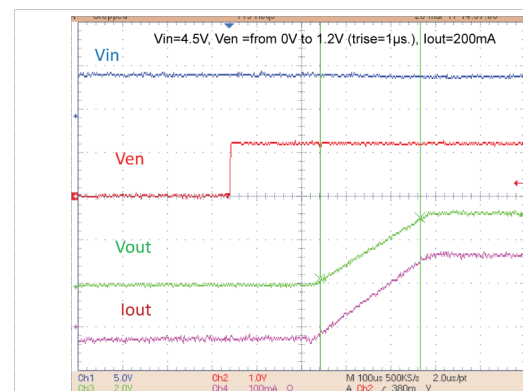
Figure 28. Enable transient
