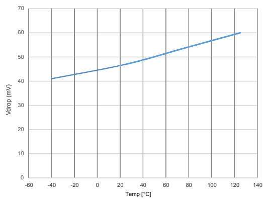
Figure 15. Dropout voltage vs. temperature I OUT = 100 mA
