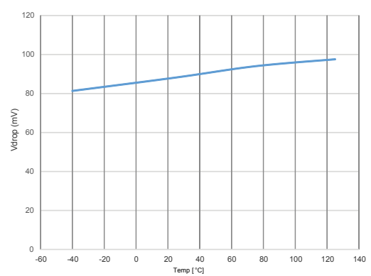
Figure 16. Dropout voltage vs. temperature I OUT = 200 mA
