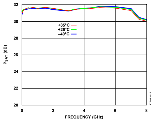
Figure 18. P_{SAT} vs. Frequency at Various Temperatures
