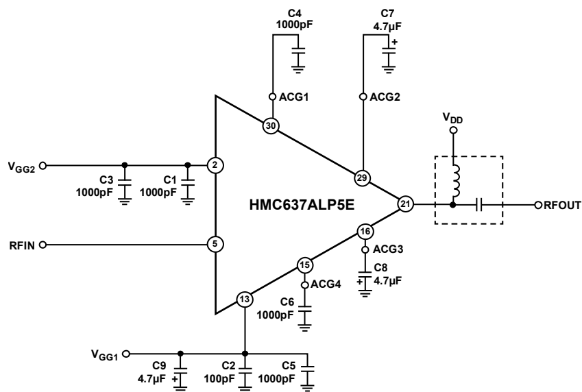
Figure 21. Application Circuit
