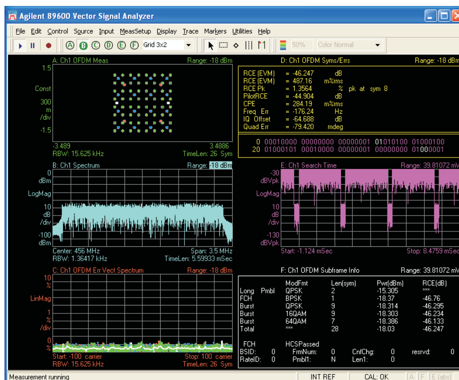
Figure 3. TRF1115EVM Performance
