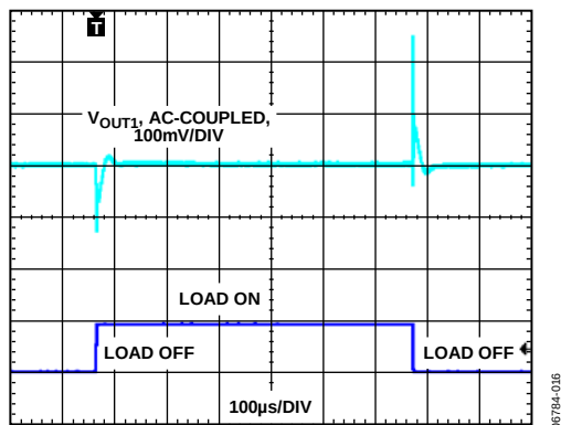
Figure 16. 1.5 A to 15 A Load Transient Response, V_{IN} = 12\text{ V}
