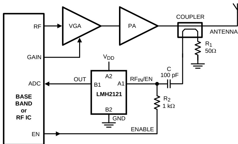
Figure 47. Transmit-Power Control System
