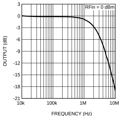
Figure 53. Response Bandwidth
