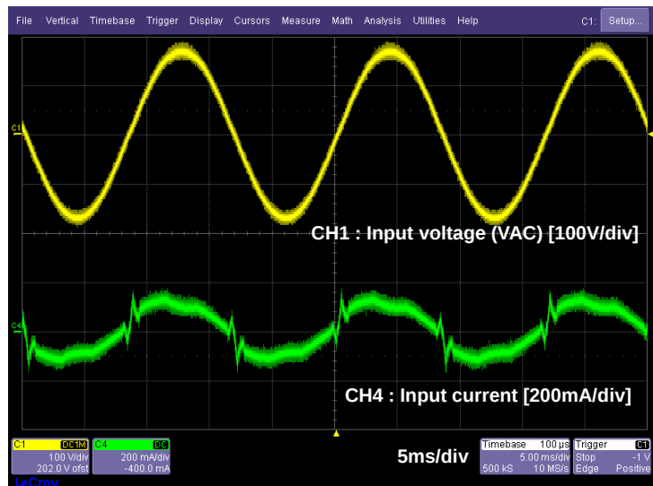
Figure6. Input waveform
