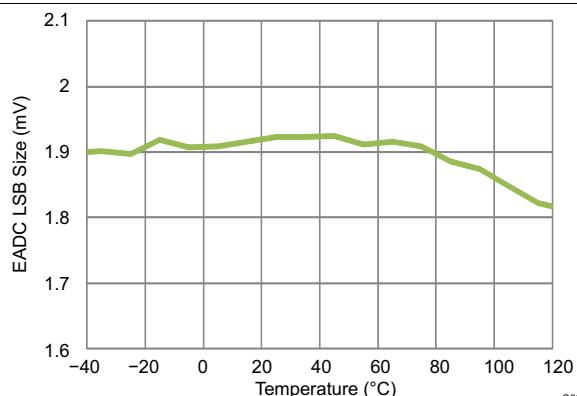
Figure 5-9. EADC LSB Size With 4X Gain (mV) vs Temperature
