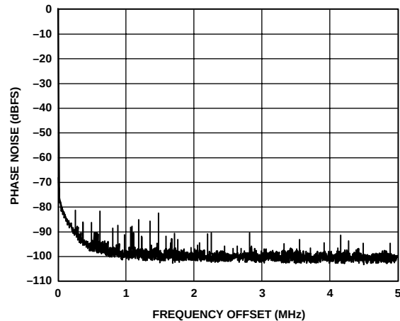
Figure 47. Phase Noise Performance
