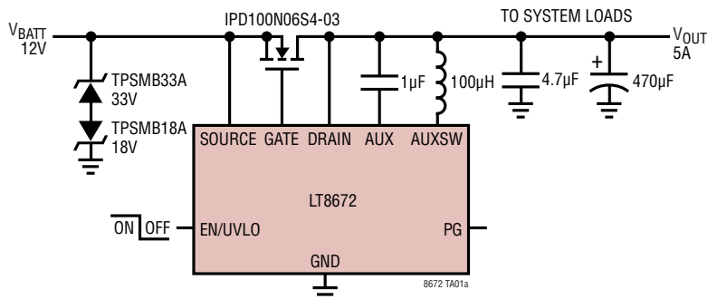
12V, 5A Automotive Reverse Battery Protection
