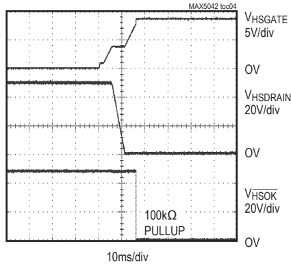
HOT-SWAP STARTUP WAVEFORM
