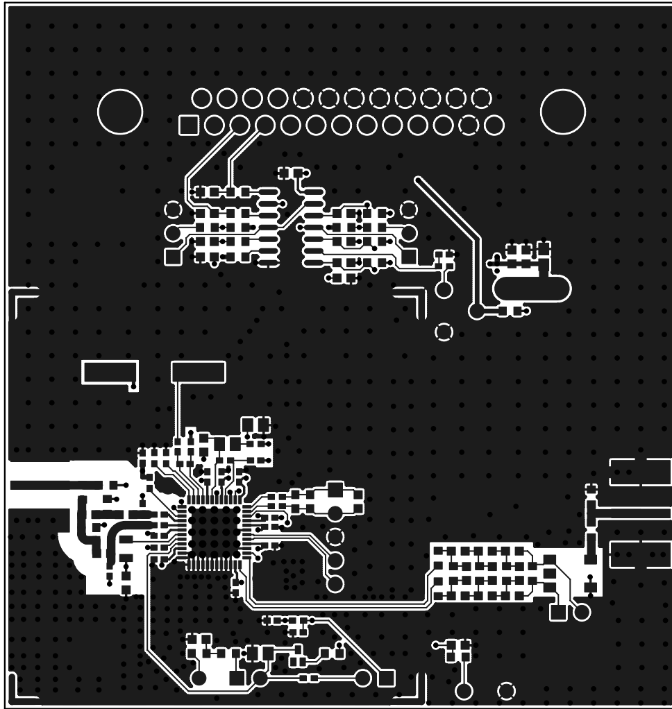
Figure 3. MAX3541/MAX3542 EV Kits PCB Layout—Primary Component Side
