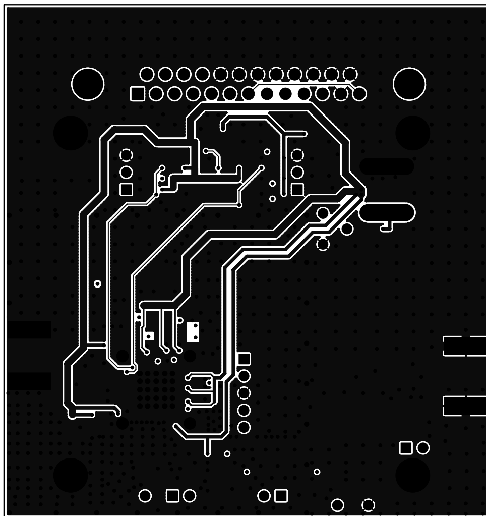
Figure 6. MAX3541/MAX3542 EV Kits PCB Layout—Secondary Component Side
