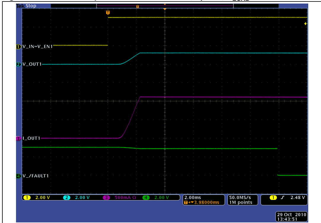
Figure 37. Overcurrent protection characteristics, V_I = 3\text{ V} , R_{LOAD} = 1\ \Omega
