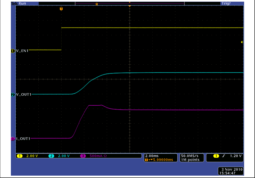
Figure 25. Turn-on for C LOAD = 470 μF
