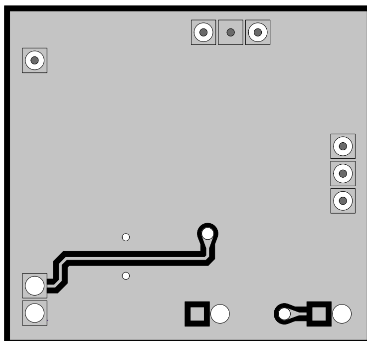
Figure 2–6. TPA2000D1 Filterless Class-D EVM Bottom Layer (Top View)
