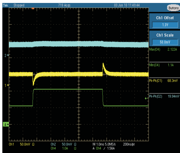
Figure 11. Buck 1 (Yellow Trace) Dynamic Response 1-A - 2-A Step, 50 mV/div. Buck 2 (Blue Trace), 50 mV/div V_{IN} = 12\text{ V} , f_{SW} = 500\text{ kHz} , L_O = 4.7\text{ }\mu\text{H} , DCR = 10 m \Omega , C_O = 22\text{ }\mu\text{F}
