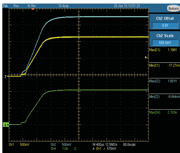
Figure 7. Soft Start for Buck 1 (Yellow Trace) 1.2 V, 3 A and Buck 2 (Blue Trace) 1.8 V, 2 A, V_{IN} = 12\text{ V} , f_{SW} = 500\text{ kHz} , L_O = 4.7\text{ }\mu\text{H} , DCR = 10\text{ m}\Omega , C_O = 22\text{ }\mu\text{F}
