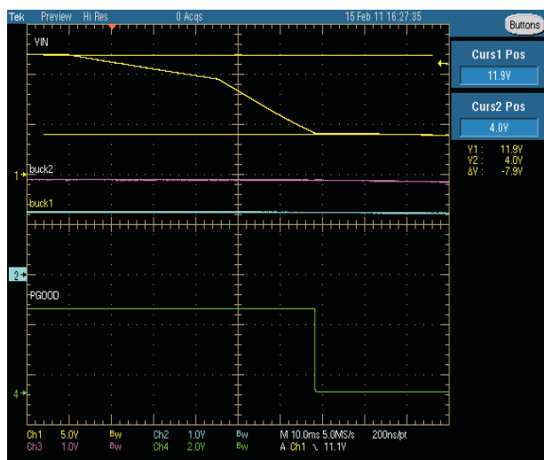
Figure 9. Power Down Behavior (From Top to Bottom V_{IN} , Buck2 = 1.8 V, Buck1 = 1.2 V, PGOOD) V_{IN} = 12\text{ V} , f_{SW} = 500\text{ kHz} , L_O = 4.7\text{ }\mu\text{H} , DCR = 10 m \Omega , C_O = 22\text{ }\mu\text{F}
