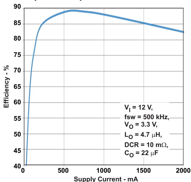
Figure 6. Buck 2 Efficiency, V_O = 3.3\text{ V} , V_{IN} = 12\text{ V} , f_{SW} = 500\text{ kHz} , L_O = 4.7\text{ }\mu\text{H} , DCR = 10\text{ m}\Omega , C_O = 22\text{ }\mu\text{F}
