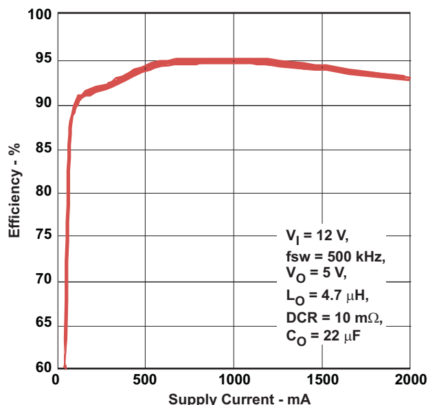
Figure 5. Buck 2 Efficiency, V_O = 5\text{ V} , V_{IN} = 12\text{ V} , f_{SW} = 500\text{ kHz} , L_O = 4.7\text{ }\mu\text{H} , DCR = 10\text{ m}\Omega , C_O = 22\text{ }\mu\text{F}
