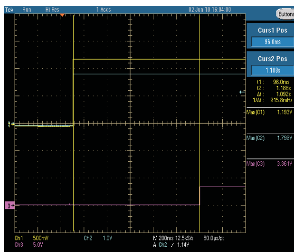
Figure 8. Power Up and PGOOD (From Top to Bottom, Buck2 = 1.8 V, Buck1 = 1.2 V, PGOOD) V_{IN} = 12\text{ V} , f_{SW} = 500\text{ kHz} , L_O = 4.7\text{ }\mu\text{H} , DCR = 10\text{ m}\Omega , C_O = 22\text{ }\mu\text{F}
