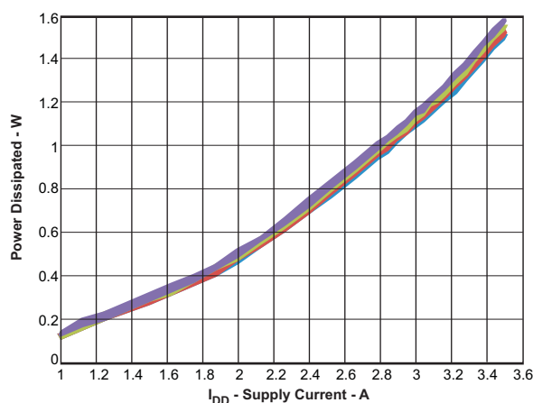
Figure 27. Buck 1 V_{IN} = 5 V, f_S = 1.1 MHz, V_O (From Top to Bottom) = 5, 3.3, 2.5, 1.8, 1.2 V
