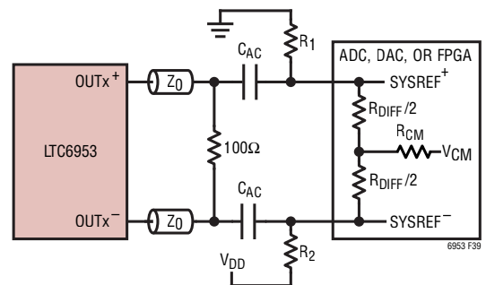
Figure 39. OUTx CML AC-Coupled Connections to SYSREF Inputs for Pulsed Mode Operation
