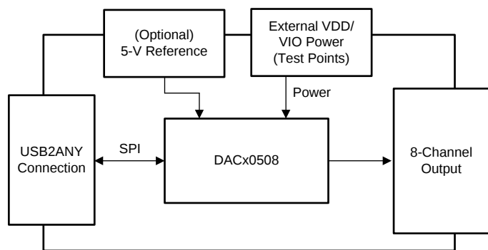
Figure 2. DACx0508EVM Block Diagram
