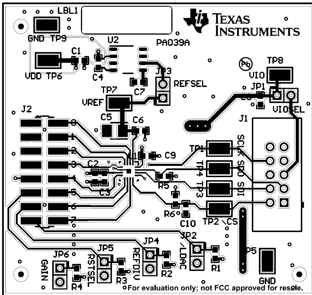
Figure 13. DACx0508EVM PCB Components Layout
