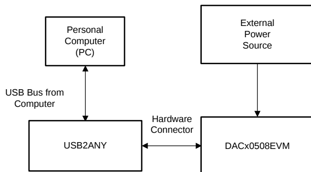
Figure 1. DACx0508EVM Hardware Setup
