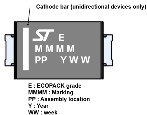
Figure 18. SMA marking
