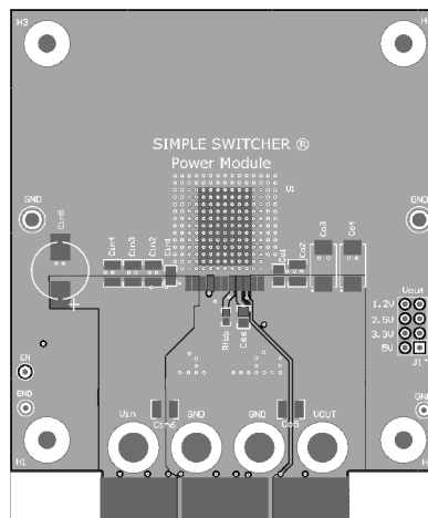
Figure 58. Top View of Evaluation PCB
