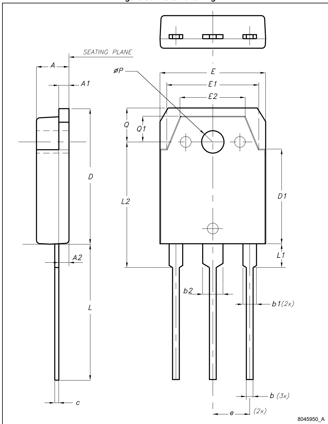
Figure 36. TO-3P drawing
