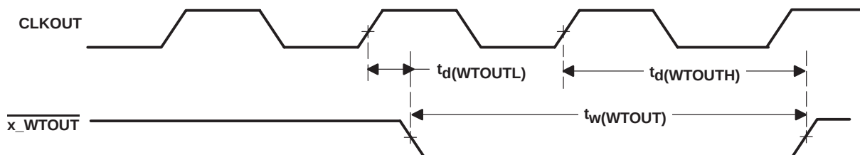
Figure 5–8. Watchdog Timer (x_WTOUT) Timing
