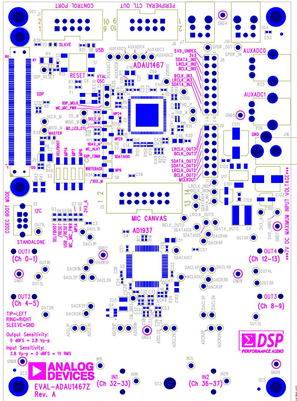
Figure 106. EVAL-ADAU1467Z Layout, Top Assembly and Silkscreen
