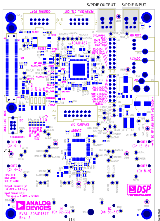
Figure 33. Location of S/PDIF Optical Input (J10) and Output (J7), Rotated 90°
