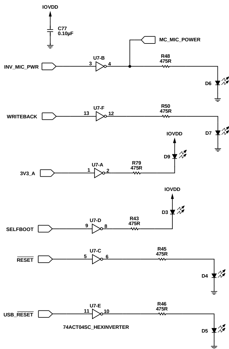
Figure 104. Status LEDs and Inverter Schematic
