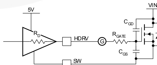
Figure 17. Drive Equivalent Circuit
