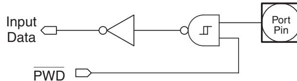
Figure 10-3. Input Circuit for P3.2, P3.3 and P3.6
