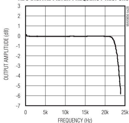
ADC DIGITAL FILTER FREQUENCY RESPONSE
