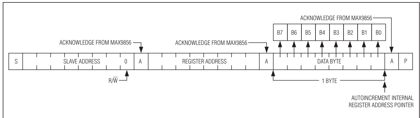
Figure 11. Writing 1 Byte of Data to the MAX9856
