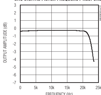
DAC DIGITAL FILTER FREQUENCY RESPONSE
