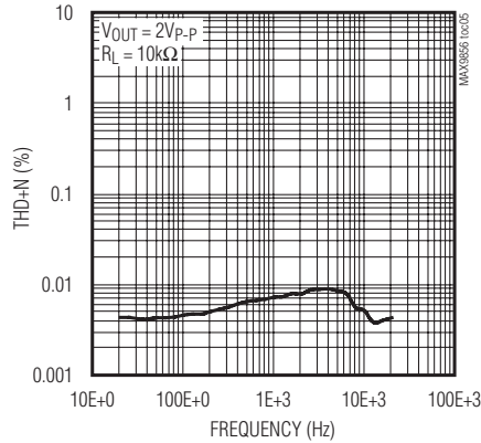
TOTAL HARMONIC DISTORTION PLUS NOISE vs. FREQUENCY (INTMIC TO ADC)
