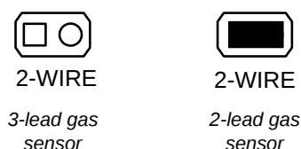
Figure 2: 2-WIRE Jumper Settings
