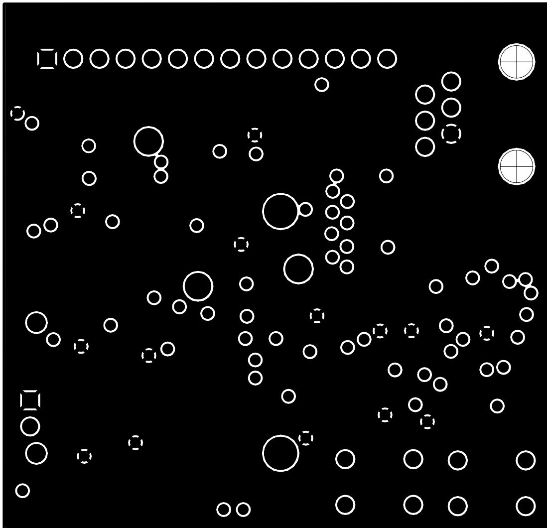
FIGURE A-7: MCP2140 IrDA® STANDARD WIRELESS TEMPERATURE SENSOR DEMO BOARD LAYOUT - POWER LAYER
