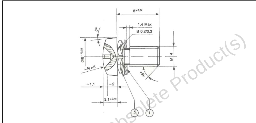
Figure 21. Mounting section
