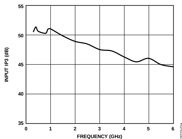
Figure 13. Input IP3 vs. Frequency at Room Temperature, V_{DD} = 5\text{ V}
