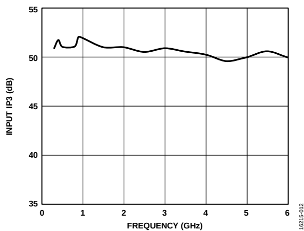
Figure 11. Input IP3 vs. Frequency at Room Temperature, V_{DD} = 3\text{ V}
